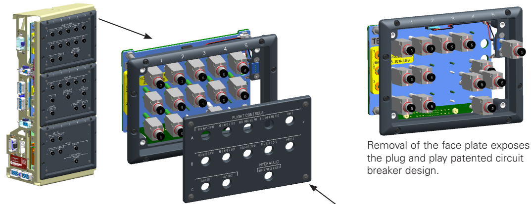
Each face plate is easily removable and is held to the module by four screws.
