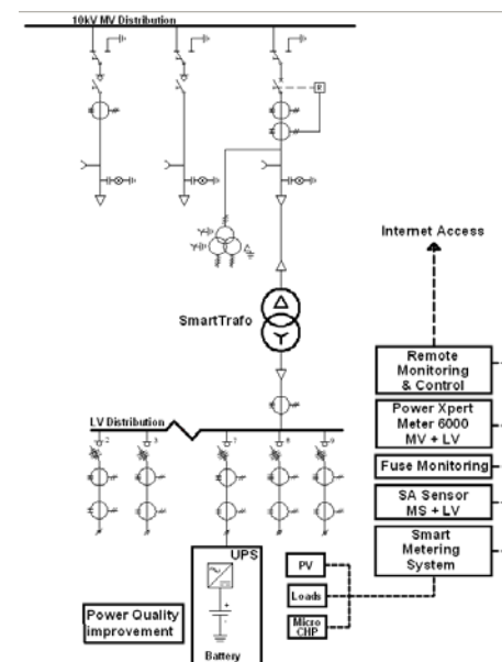
Figure 3 Electrical circuit diagram
