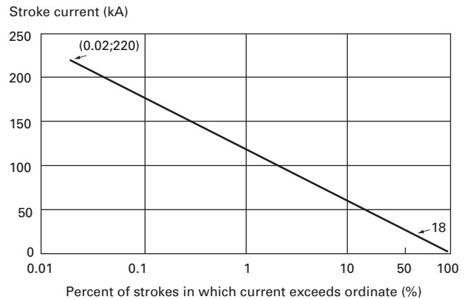
FIGURE 9. DISTRIBUTION OF LIGHTNING STROKE CURRENTS ①
