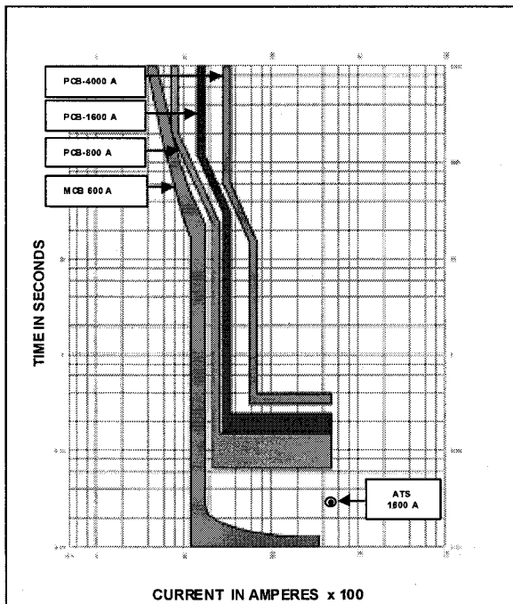
Fig. 3. System Time-Current Coordination
