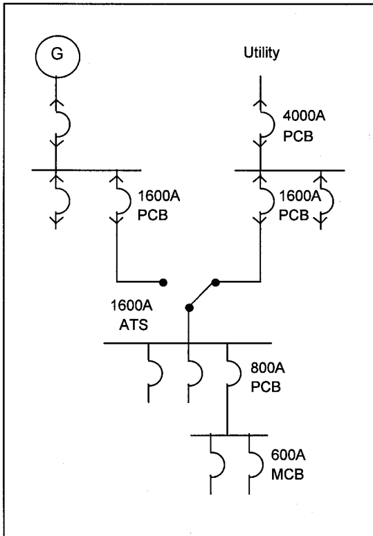
Fig. 2. System One-Line Diagram
