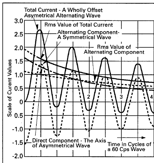
Fig. 1. Structure of an Asymmetrical Current Wave
