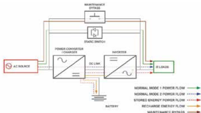
Figure 3. Internal design of a multi-mode UPS.
