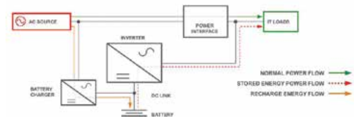
Figure 1. Internal design of a line-interactive UPS.
