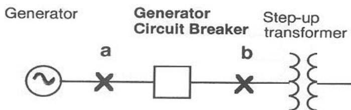
FIGURE 1. Typical Generator Circuit [1]
