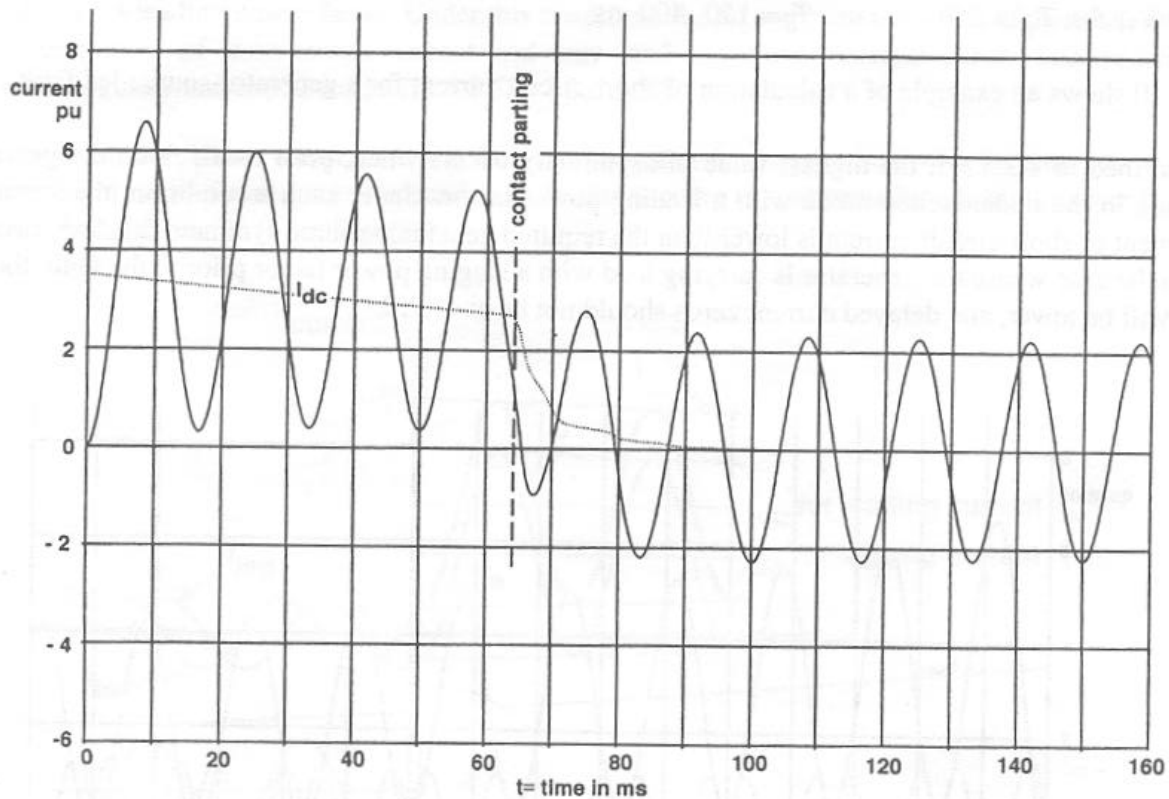
FIGURE 2. Short-circuit Current with Delayed Current Zeroes [1]
