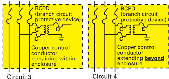
Figure 7.14.8.e Control circuit conductor 14 AWG and larger protection.
