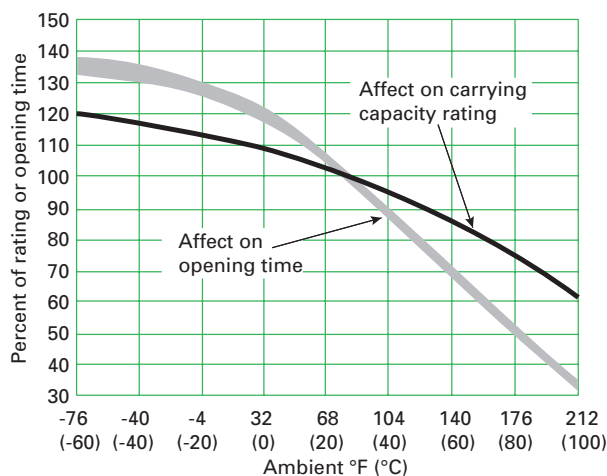
Figure 3.1.3.2.i Ambient temperature dual-element fuse derating curve.
