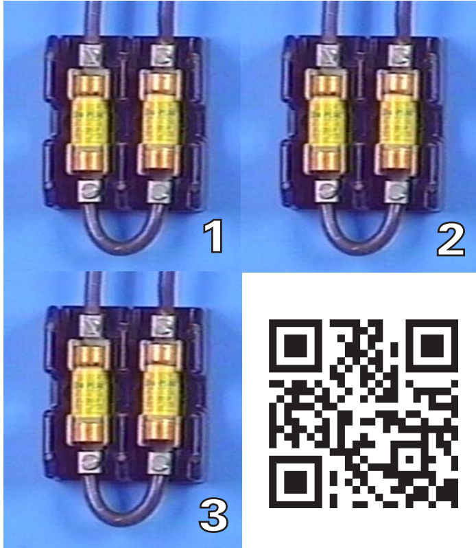
Figure 3.1.4.3.f A fuse applied within its interrupting rating.
