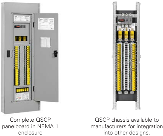
8.1.8.2.b Quik-Spec Coordination Panelboard (QSCP).
