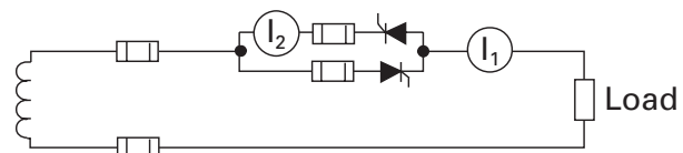
Figure 3.1.6.4.g Single-phase, anti-parallel, AC control.
