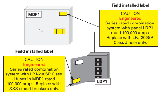
Figure 7.6.5.a Existing installation labeling per 240.86(A) and 110.22(B).
