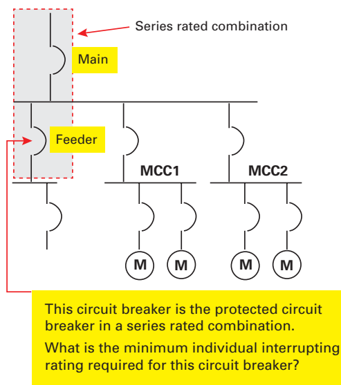
Figure 7.6.7.a Example 1 diagram.
