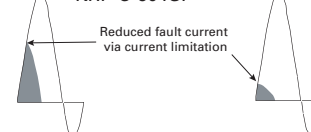
Test 3: current limiting KRP-C-601SP Test 1: current limiting LPS-RK-30SP
