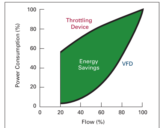
Figure 2. The Amount of Energy Saved by Using a Variable Frequency Drive (versus a Valve) to Control Flow
