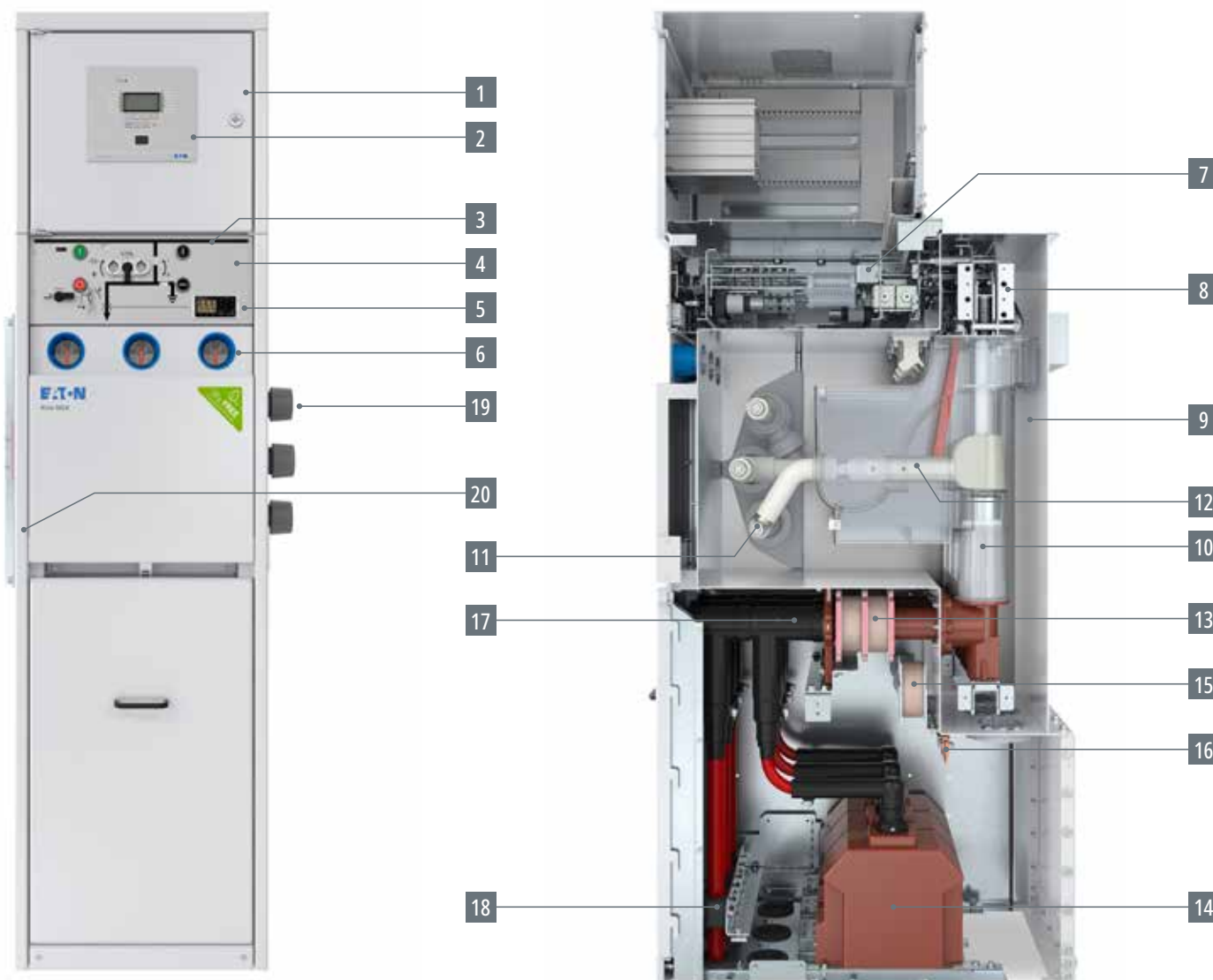
Circuit breaker panel (example)
