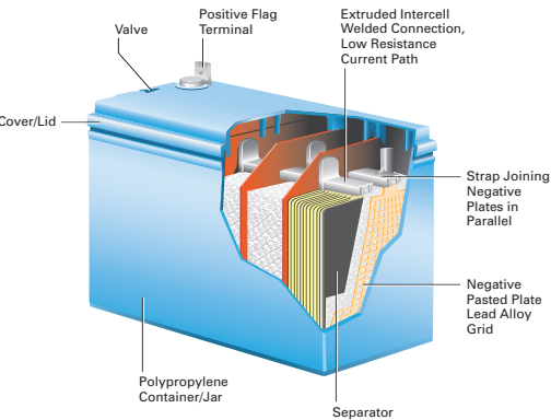
Figure 2. Internal and external components of a valve-regulated lead acid (VRLA) battery.
