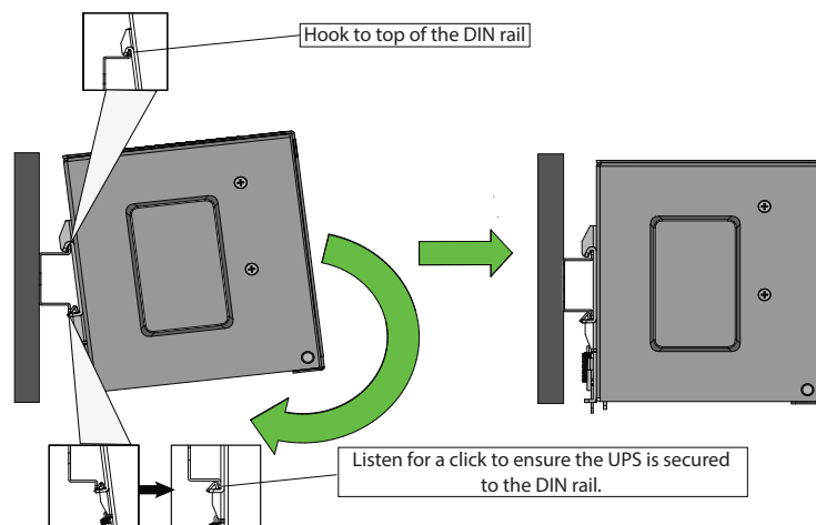
Figure 4. Mounting the BPDIN24XL EBM
