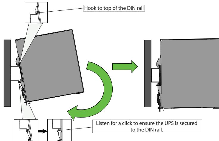
Figure 3. Mounting the UPS
