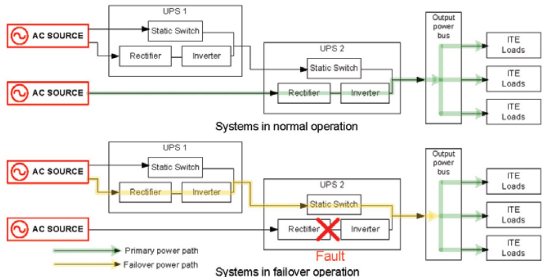
Figure 6. Serial (cascade) UPS architecture with changing power path if the UPS under load fails.
