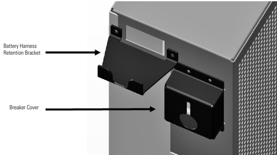
Figure 1. Battery Harness Retention Bracket and Breaker Cover
