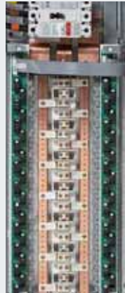
CT strip-mounted panel board
