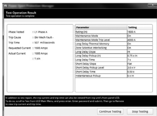
Figure 26.2-5. Example of a Completed Secondary Injection Test
