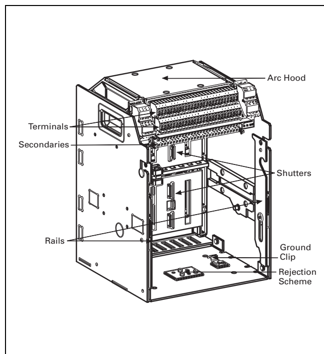
Figure 26.2-16. Cassette/Cradle Components
