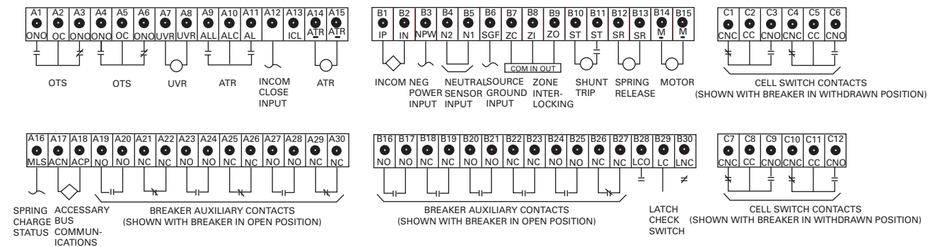
Figure 26.1-10. Typical Magnum Secondary Terminal Block Connection Diagram
