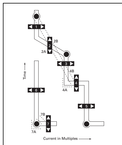
Figure 26.1-7. Time-Current Curve Shaping
