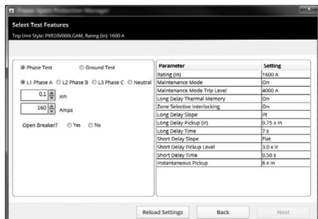
Figure 26.2-4. PXP Secondary Injection Setup
