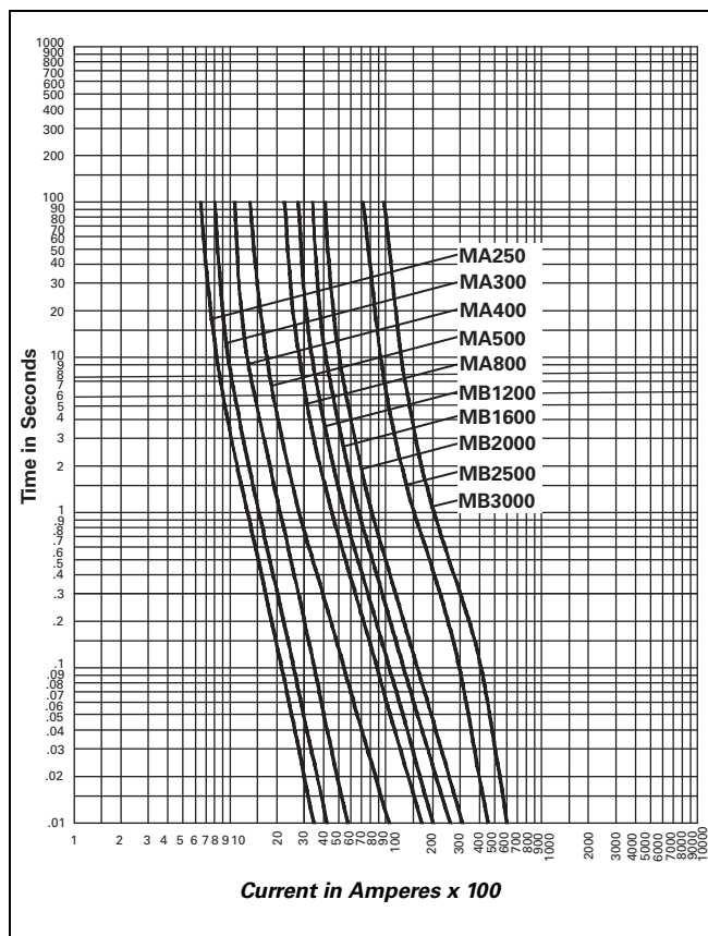
Figure 26.1-4. Type Magnum DSL Limiters Average Melting Time-Current Characteristics
