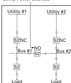
Figure 27.3-7. Circuit Breaker Fed from Multiple Power Supply Sources
