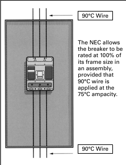
Figure 27.2-3. Conductor Requirements
