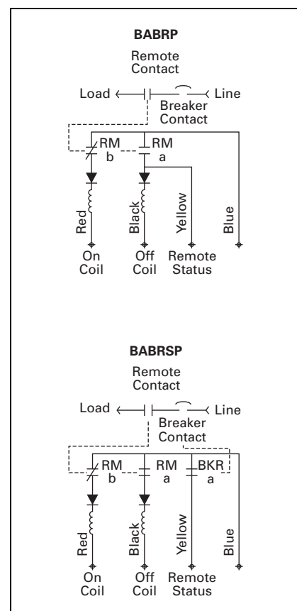
Figure 27.4-1. Control Circuit for the BABRP and BABRSP
