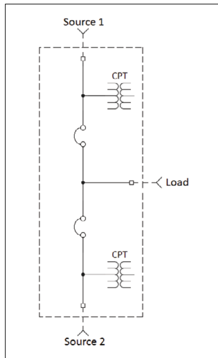
Figure 25.3-1. Power Frame Transfer Switch—Fixed
