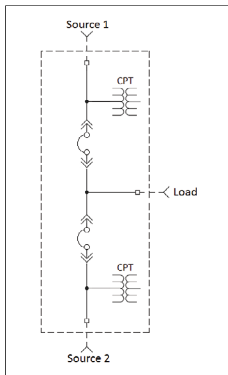
Figure 25.3-2. Power Frame Transfer Switch—Drawout
