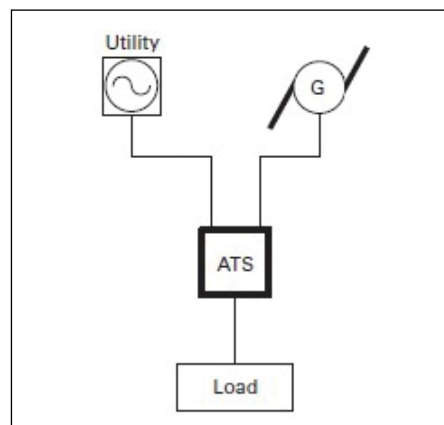
Figure 25.3-12. Utility—Generator
