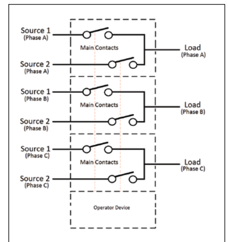
Figure 25.3-18. Switching Mechanism
