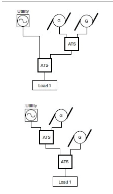
Figure 25.3-15. Utility—Generator—Generator
