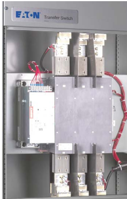
Fixed Mounting
