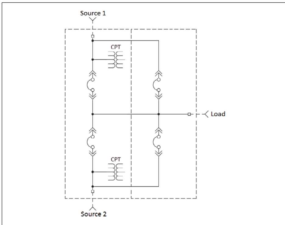
Figure 25.3-3. Power Frame Bypass Isolation Transfer Switch—Drawout
