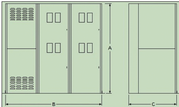
Figure 25.3-10. NEMA 1 (4000–5000 A)
