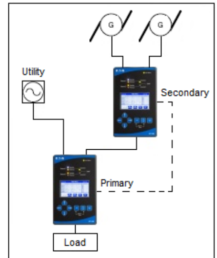
Primary/Secondary Configuration with ATC-900
