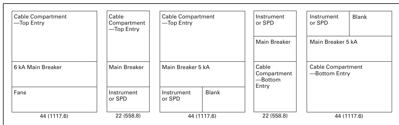
Figure 21.5-4. Front-Access Main Sections
