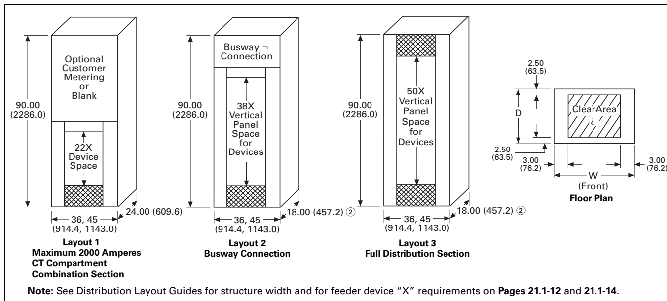
Figure 21.1-7. Distribution Section Layouts—Dimensions in Inches (mm)
