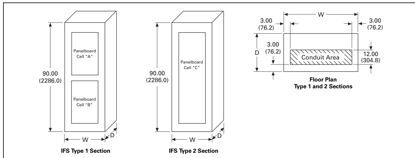
Figure 21.6-4. Type 1 and 2 Integrated Facility System Switchboards Distribution Section Layout—Dimensions in Inches (mm)
