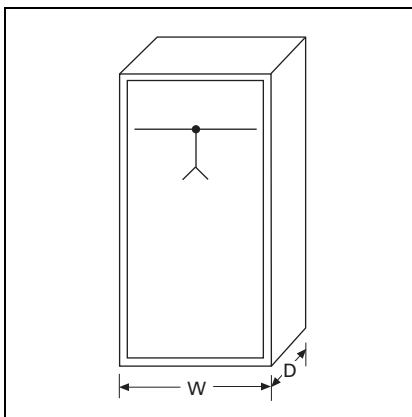
Figure 21.10-10. Main Lug Only—Top or Bottom Feed
