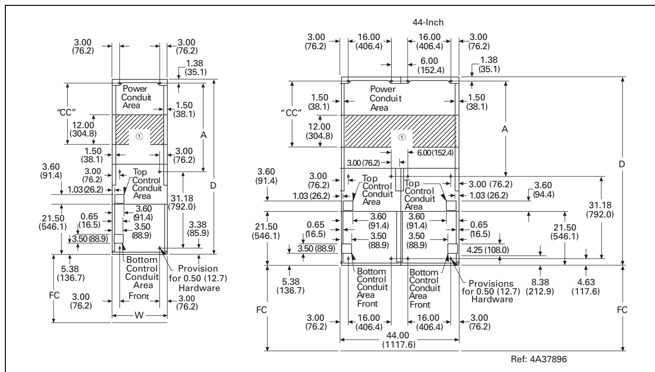
Figure 21.5-10. Floor Plans and Available Conduit Space in Inches (mm)—18.00, 22.00, 30.00, 44.00-Inch (457.2, 558.8, 762.0, 1117.6 mm) Wide Rear-Access Structures
