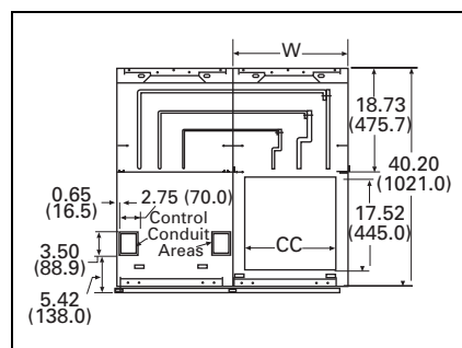
Figure 21.5-11. Front- Access Structures
