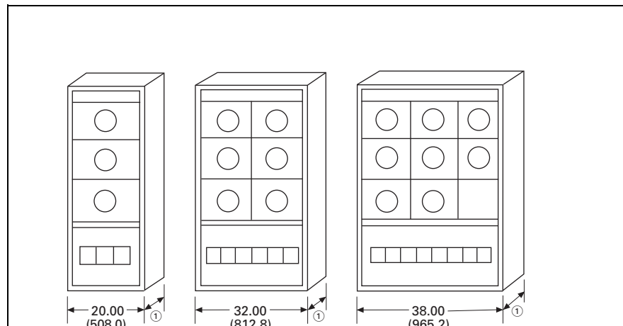
Figure 21.10-14. Circuit Breaker or Fusible Pullout Tenant Disconnects
