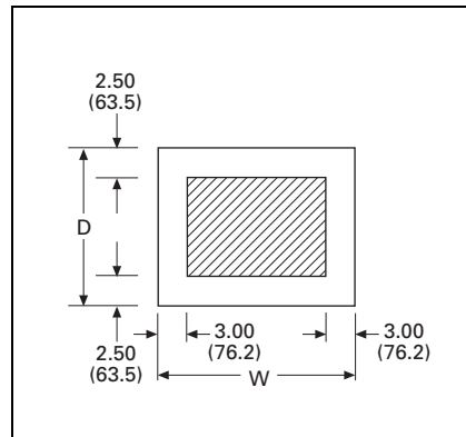
Figure 21.10-6. Typical Conduit Area
