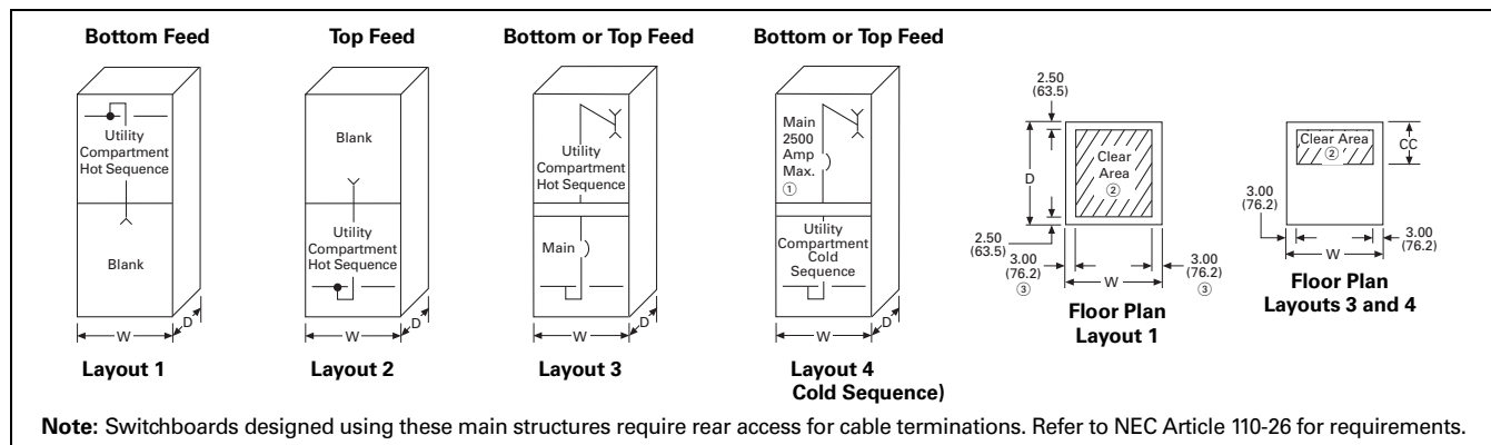
Figure 21.2-1. Utility Compartment Layouts—Dimensions in Inches (mm)
