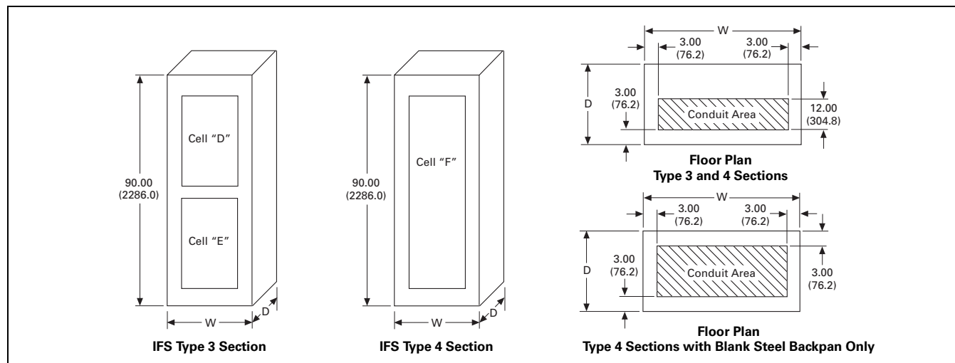
Figure 21.6-5. Type 3 and 4 Integrated Facility System Switchboards Distribution Section Layout—Dimensions in Inches (mm)
