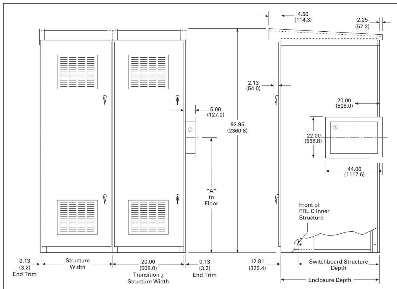
Figure 21.4-2. Front-Access—Non-Walk-In with Sloped Roof—Dimensions in Inches (mm)
