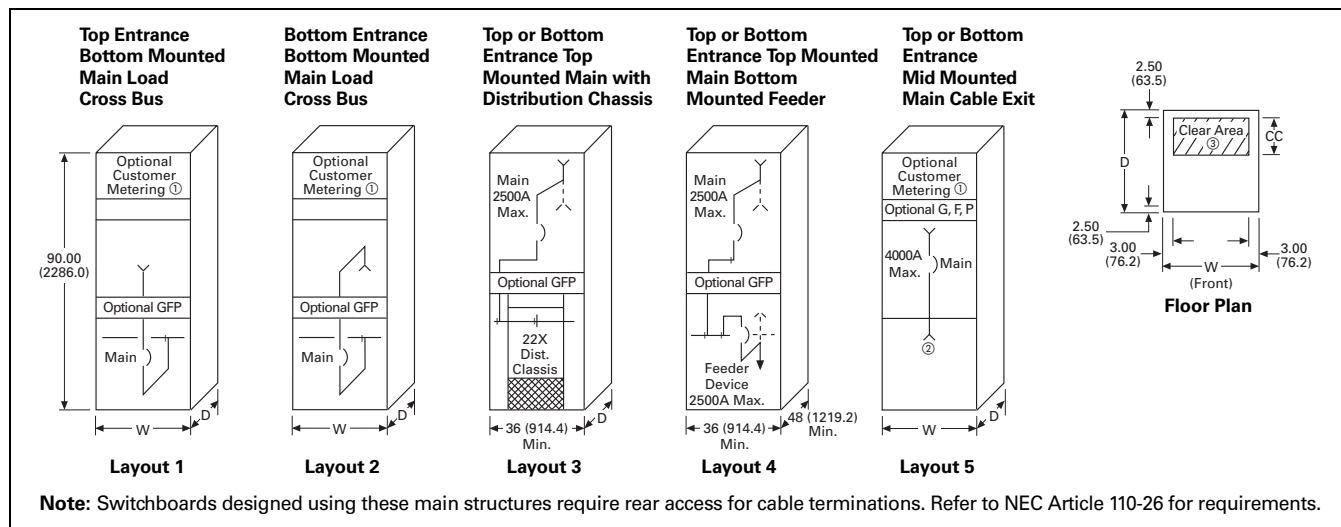
Figure 21.2-6. Main Section Layouts—Dimensions in Inches (mm)
