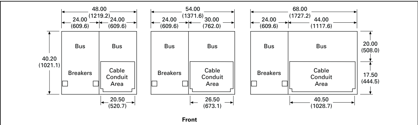
Figure 21.5-8. Floor Plans and Available Conduit Space in Inches (mm)—Front-Access Structures
