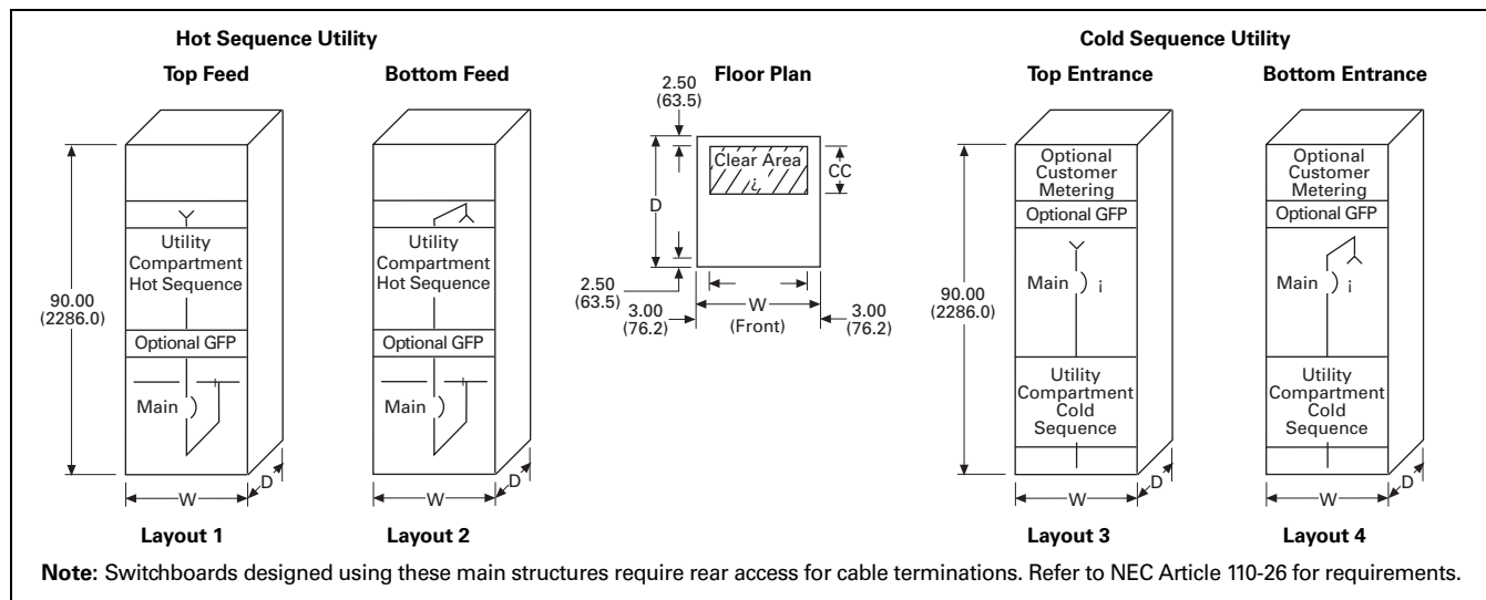
Figure 21.2-4. NEMA Utility Compartment Layouts—Dimensions in Inches (mm)
