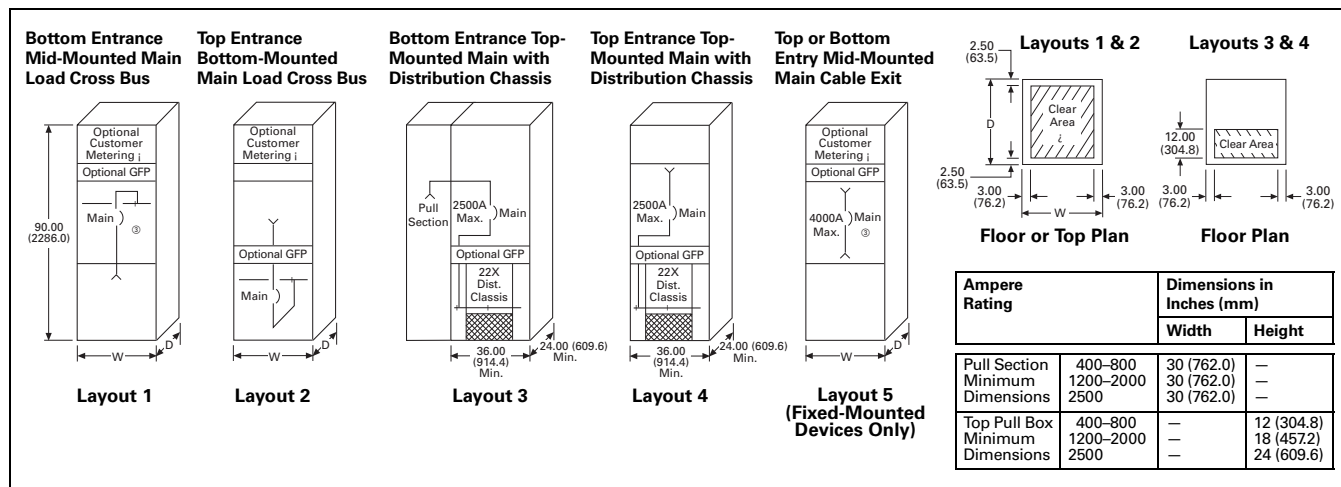
Figure 21.1-5. Main Structure Layouts—Dimensions in Inches (mm)
