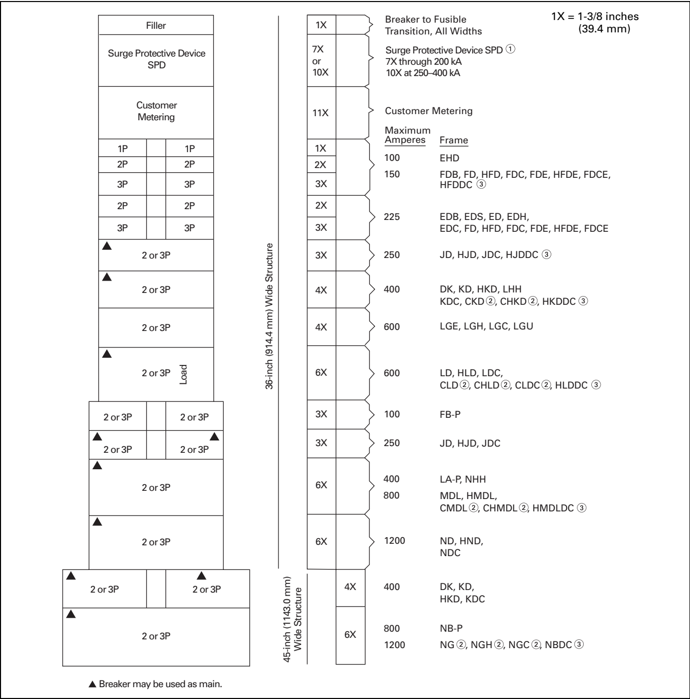
Figure 21.2-11. Circuit Breaker "X" Space Requirement—Dimensions in Inches (mm)
