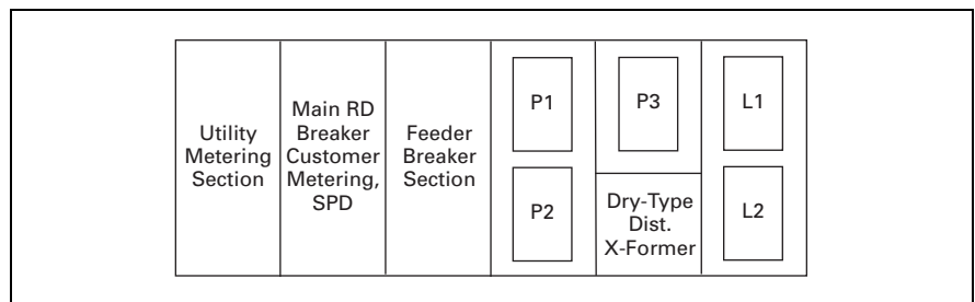
Figure 21.6-3. Optimized IFS Layout—Front View
