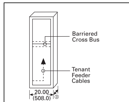
Figure 21.10-17. Load Side Pull Section with Barrired Cross Bus
