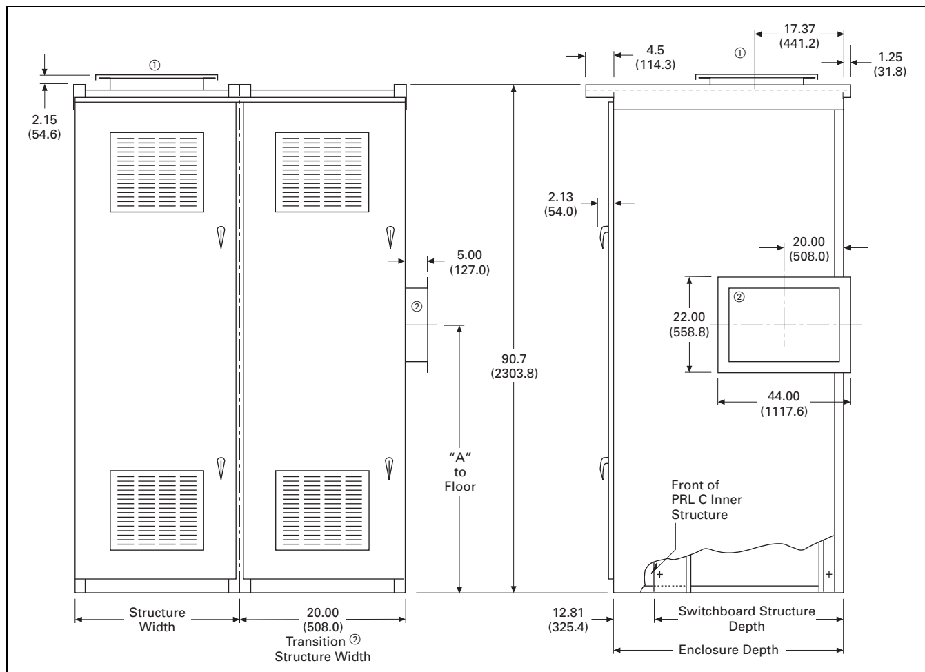
Figure 21.4-1. Front-Access—Non-Walk-In with Flat Roof—Dimensions in Inches (mm)
