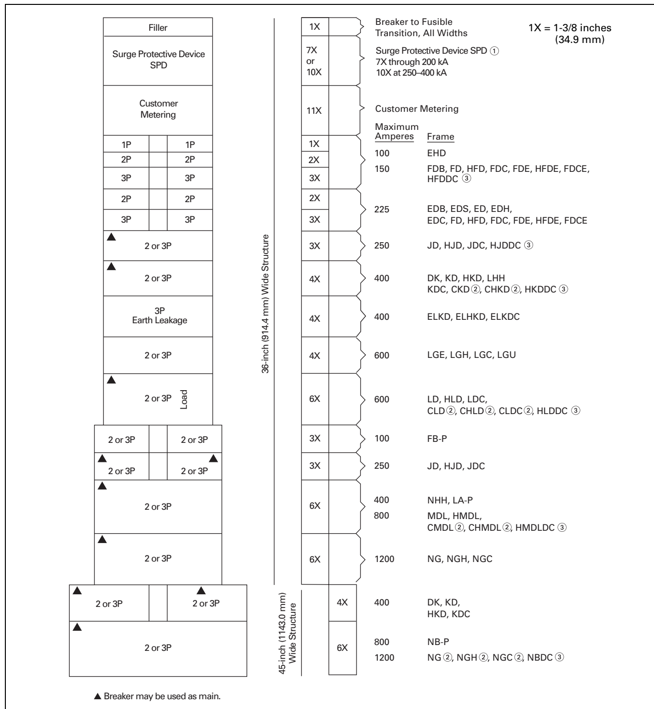
Figure 21.1-9. Circuit Breaker “X” Space Requirements—Dimensions in Inches (mm)
