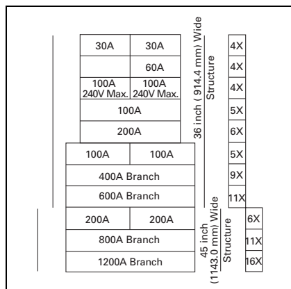
Figure 21.10-22. 22X Chassis Layout Guide—Fusible Switches
