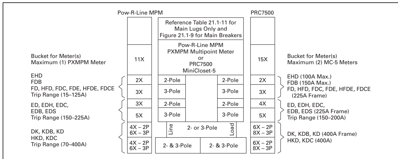
Figure 21.9-3. PRL MPM / PRC7500 Layout Guide for Current Sensor and Current Transformer Sizing—Standard Pow-R-Line C Switchboard Construction Applies
