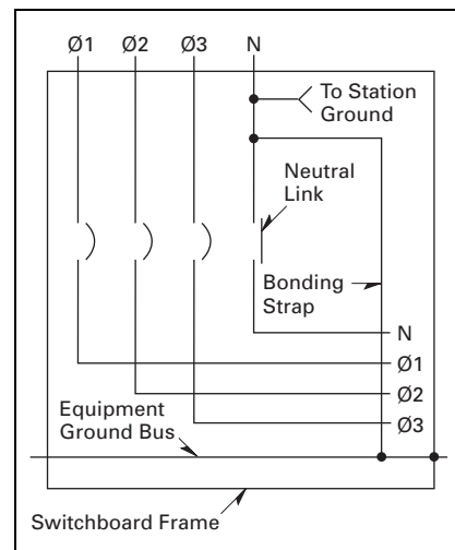
Figure 21.0-1. Neutral Link
