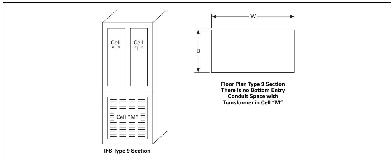
Figure 21.6-8. Type 9 Integrated Facility System Switchboards Distribution Section Layout—Dimensions in Inches (mm)
