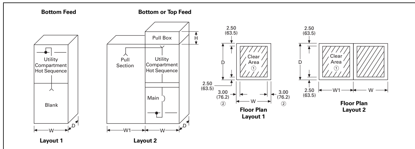
Figure 21.1-3. West Coast Utility Compartment Layouts—Dimensions in Inches (mm)
