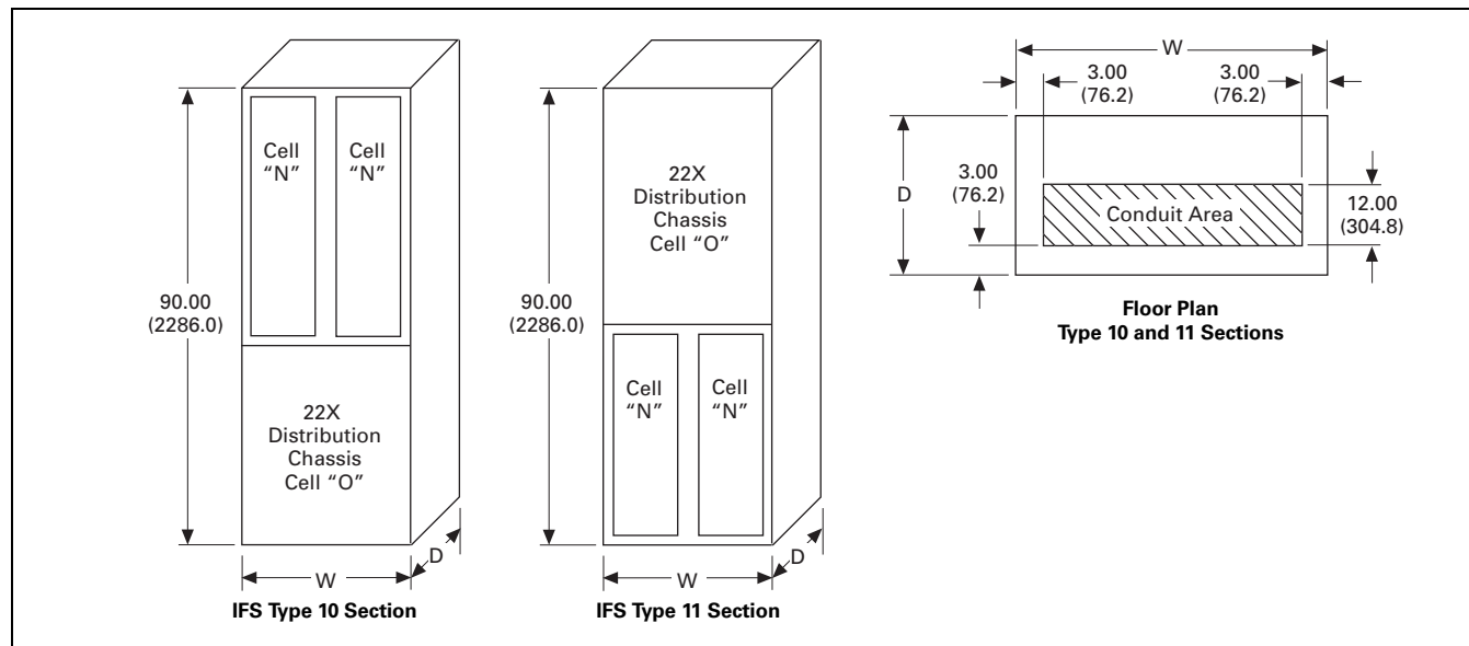
Figure 21.6-9. Type 10 and 11 Integrated Facility System Switchboards Distribution Section Layout—Dimensions in Inches (mm)
