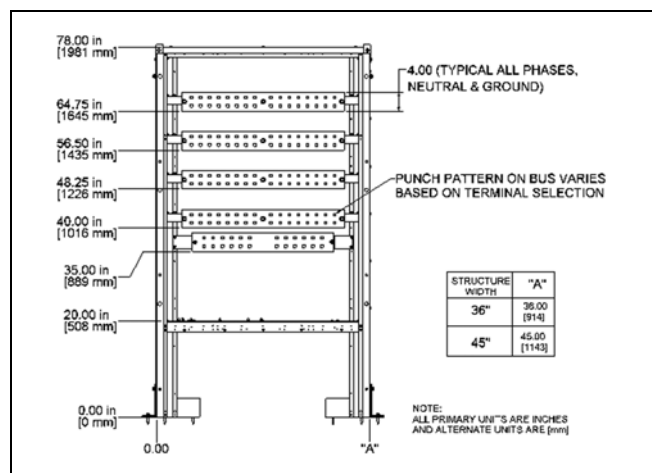
Figure 21.8-2. Front Bus Arrangement
