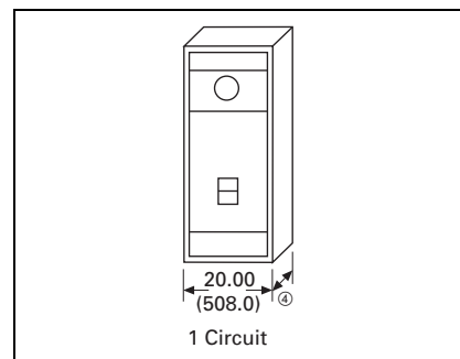
Figure 21.10-19. 400 A Tenant Section with Self-Contained Metering (Breaker)
