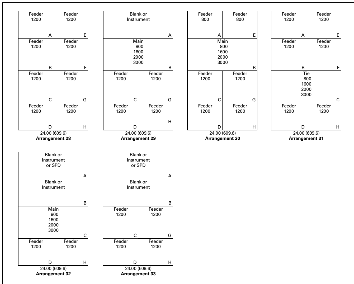
Figure 21.5-6. Typical Structure and Breaker Arrangements (Continued)—Magnum SB Mains and Ties, and Series NRX Feeder Breakers—Dimensions in Inches (mm)
