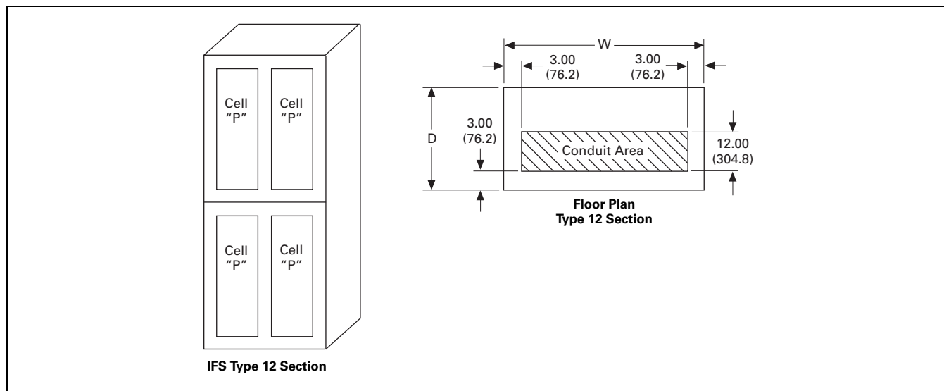
Figure 21.6-10. Type 12 Integrated Facility System Switchboards Distribution Section Layout—Dimensions in Inches (mm)
