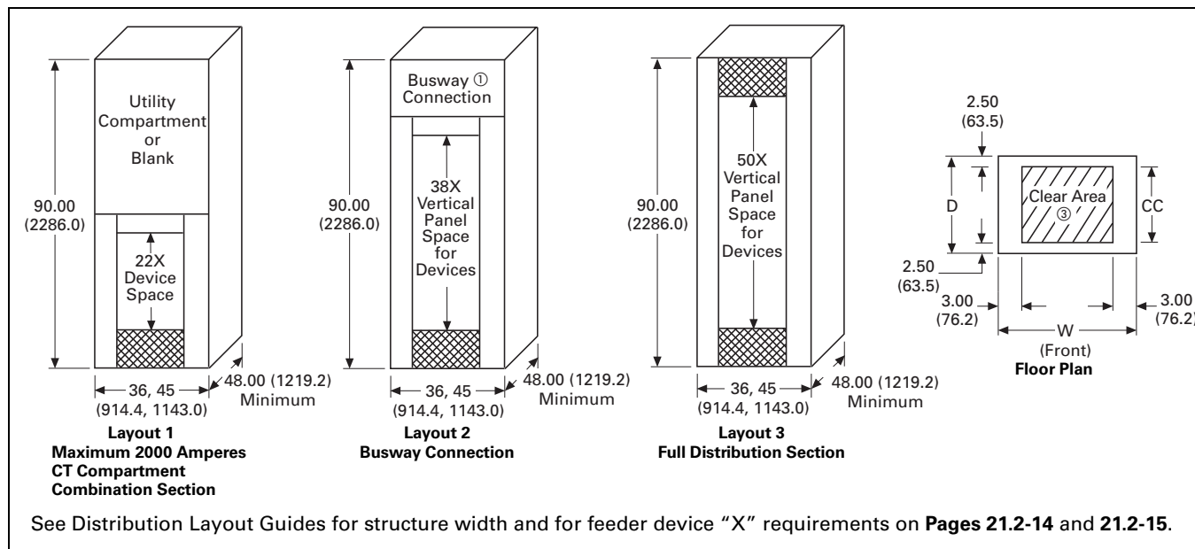
Figure 21.2-10. Distribution Section Layout—Dimensions in Inches (mm)
