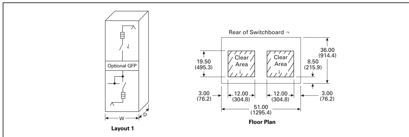
Figure 21.1-12. Individually Mounted Feeder Layout—Dimensions in Inches (mm)
