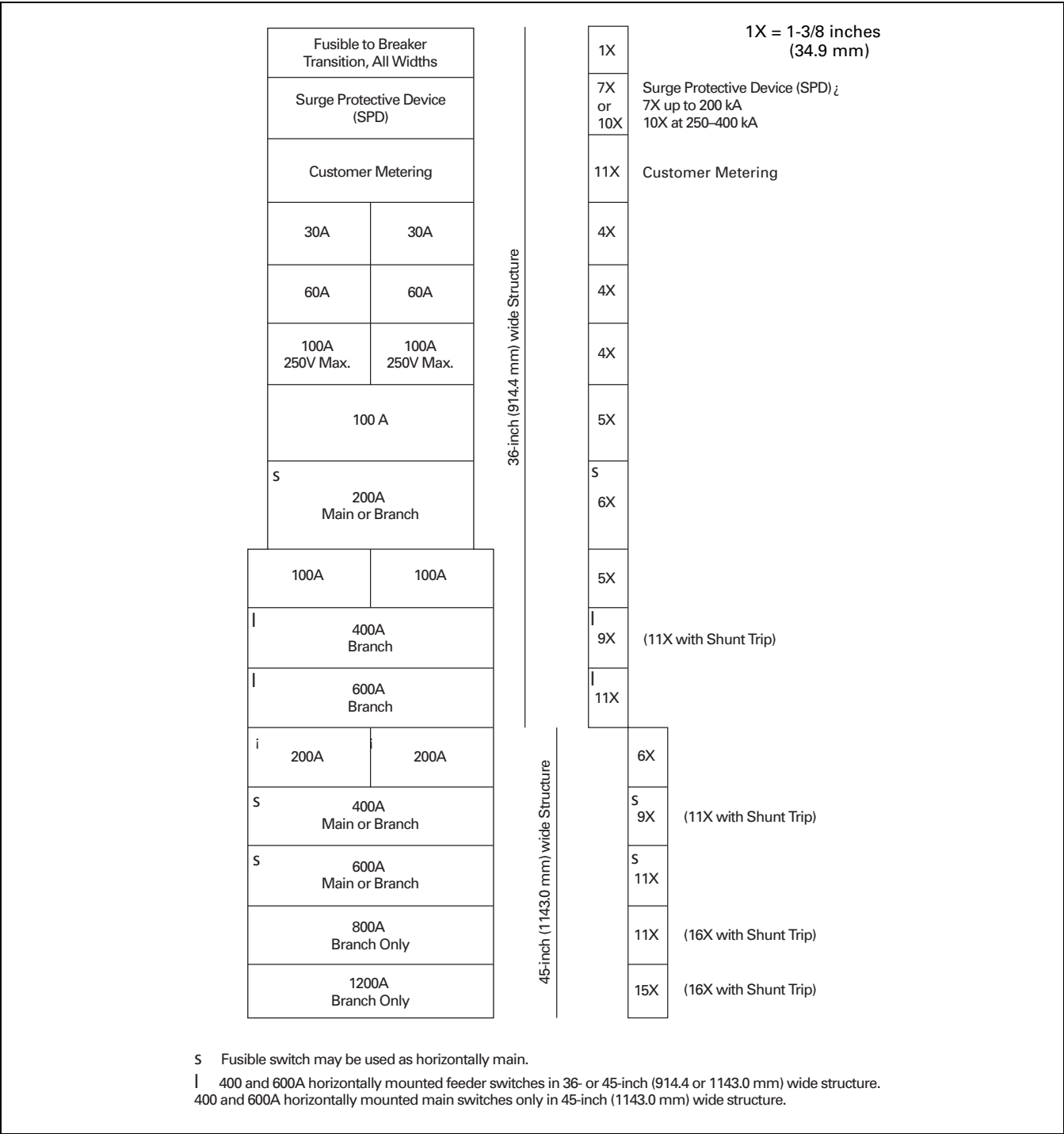
Figure 21.1-11. Fusible Switch “X” Space Requirements—Dimensions in Inches (mm)
