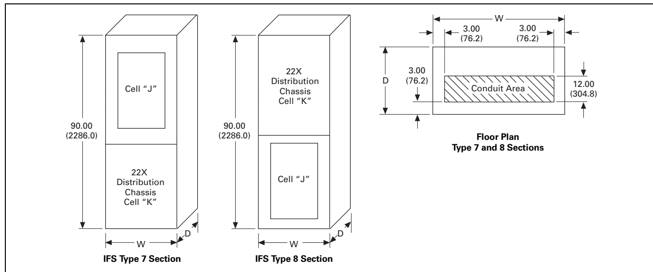
Figure 21.6-7. Type 7 and 8 Integrated Facility System Switchboards Distribution Section Layout—Dimensions in Inches (mm)
