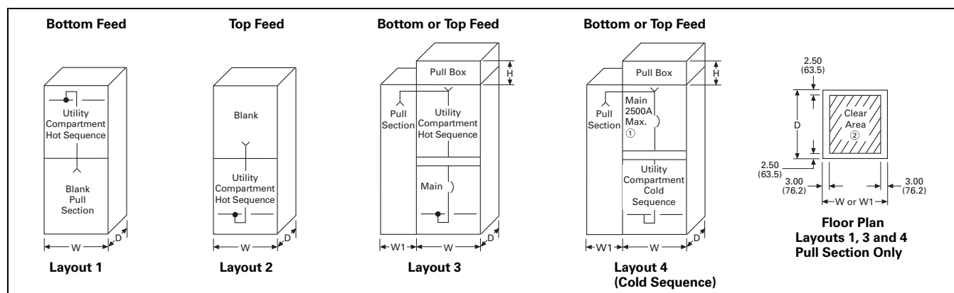
Figure 21.1-2. Incoming Utility Compartment and/or Main Devices—Dimensions in Inches (mm)
