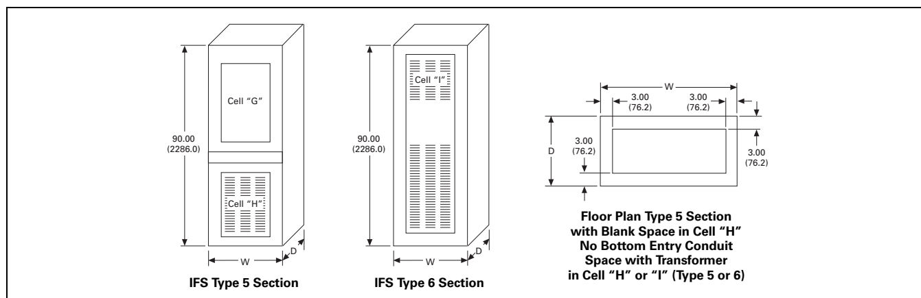
Figure 21.6-6. Type 5 and 6 Integrated Facility System Switchboards Distribution Section Layout—Dimensions in Inches (mm)
