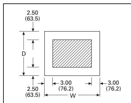
Figure 21.10-16. Typical Conduit Area—Figures 21.10-17, 21.10-18 and 21.10-19
