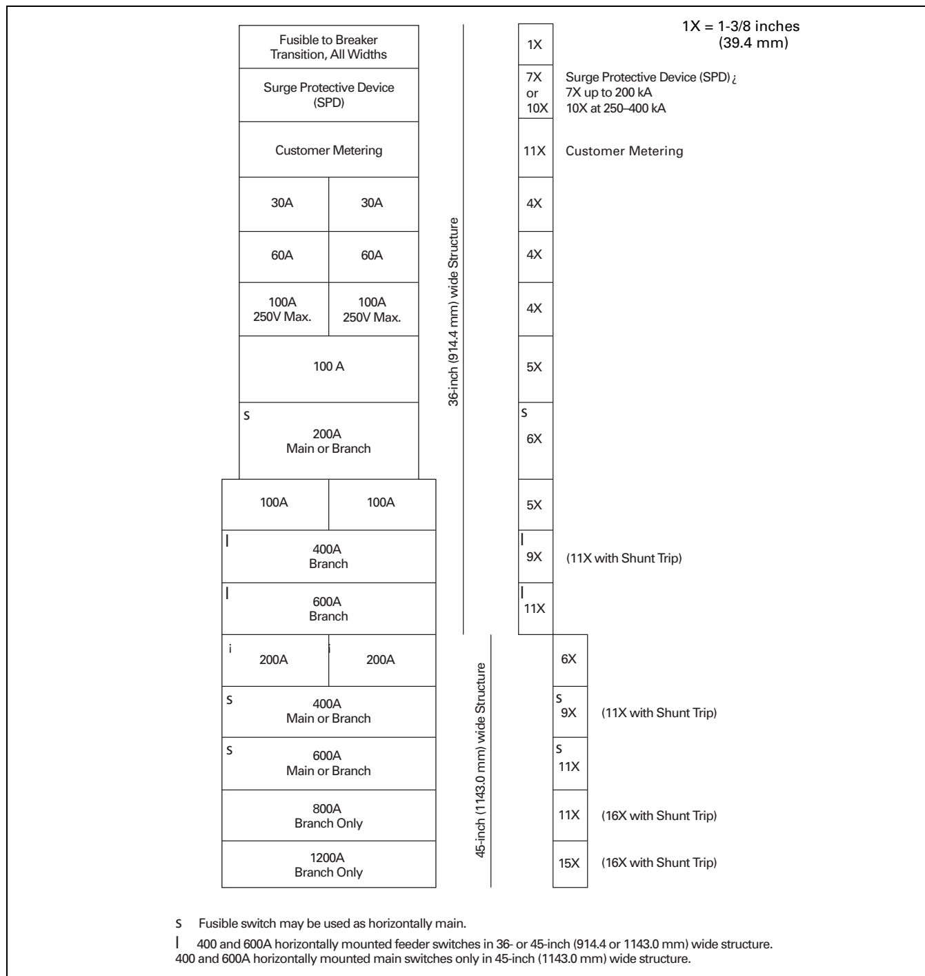
Figure 21.2-12. Fusible Switch "X" Space Requirement—Dimensions in Inches (mm)
