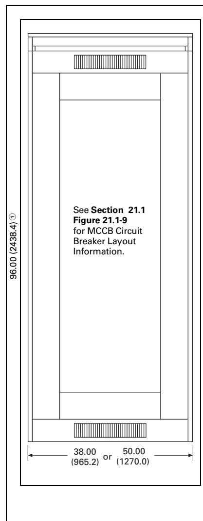
Figure 21.5-9. Group-Mounted Molded Case Circuit Breaker Switchboard
