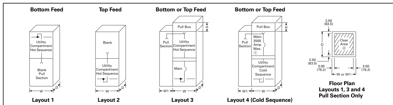
Figure 21.1-1. Incoming Utility Compartment—Dimensions in Inches (mm)
