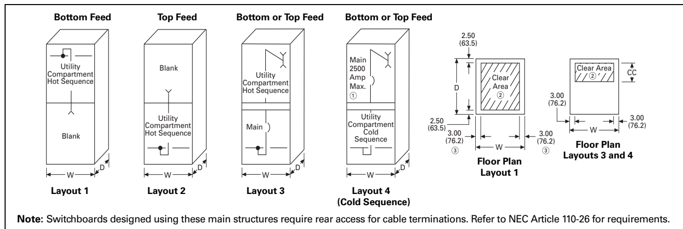
Figure 21.2-2. Utility Compartment Layouts—Dimensions in Inches (mm)
