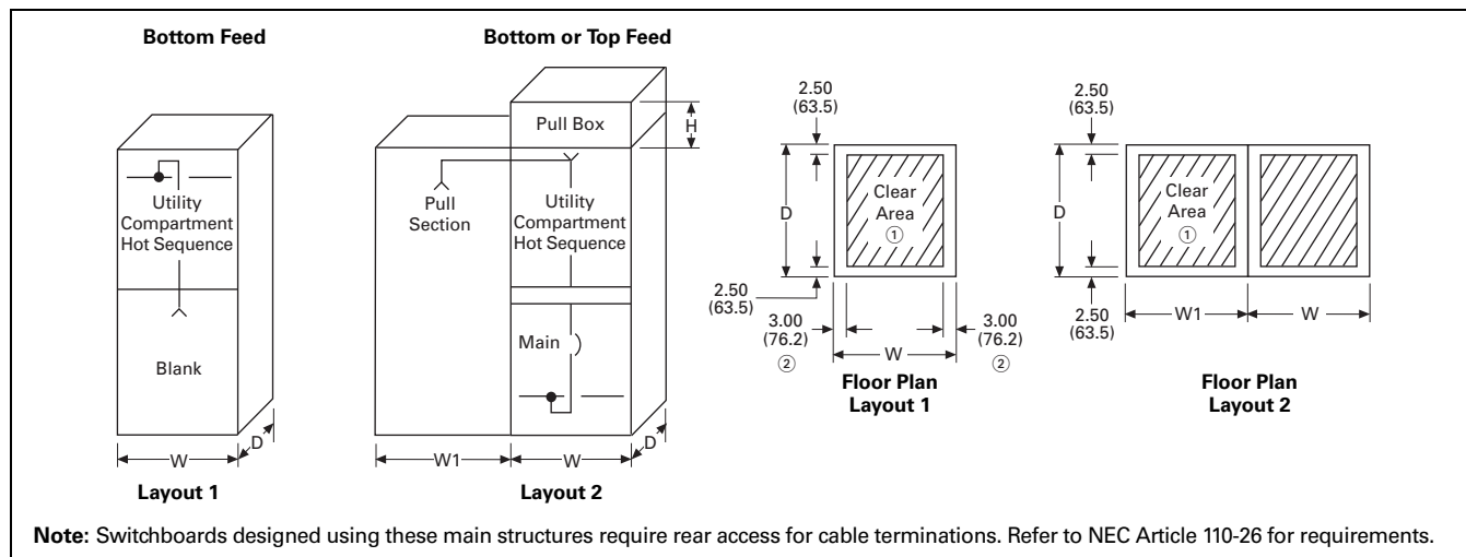
Figure 21.2-3. West Coast Utility Layouts—Dimensions in Inches (mm)
