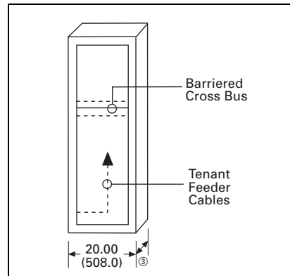
Figure 21.10-7. Load Side Pull Section with Barriered Cross Bus
