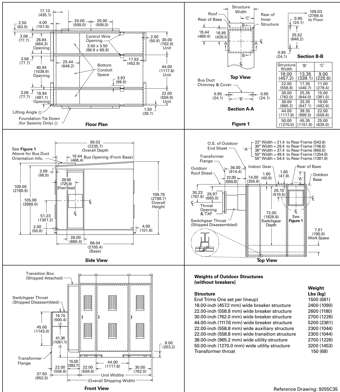
Figure 21.5-13. Outdoor Non-Walk-in Enclosure Dimensions in Inches (mm)
