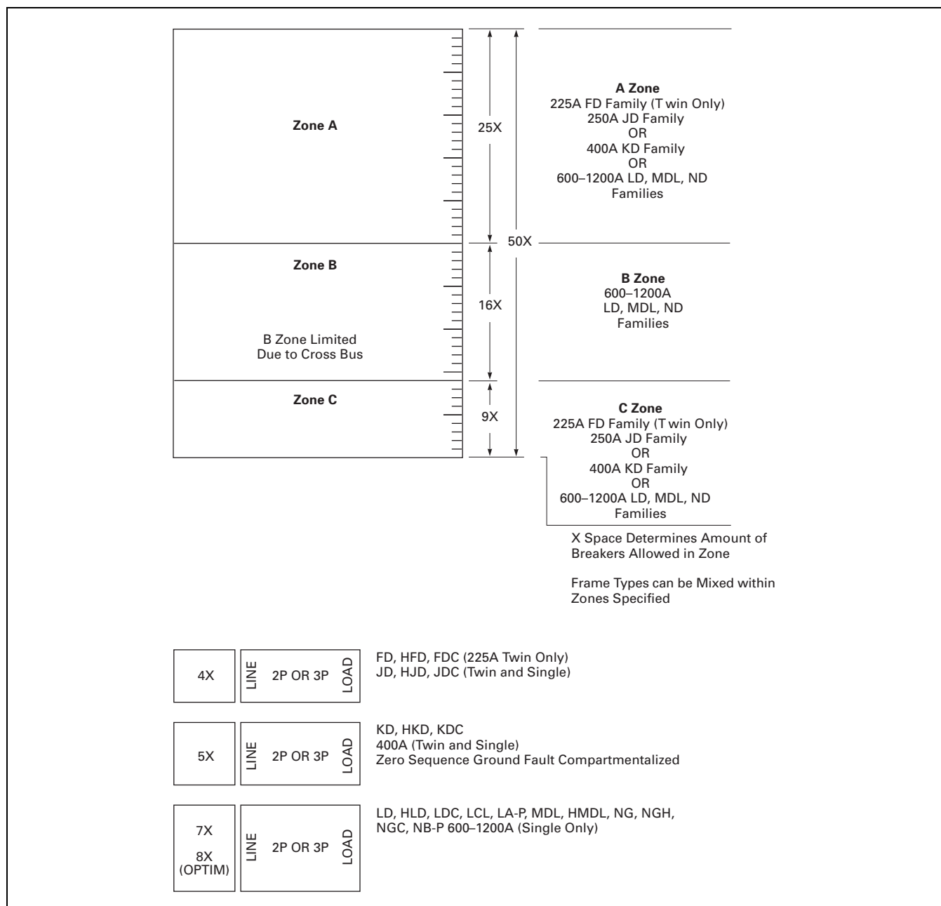
Figure 21.3-1. Individually Compartmentalized Feeder Layout 36.00-Inch (914.4 mm) Wide Section 50X Structure Only (4000 A Maximum)
