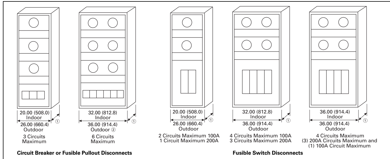
Figure 21.10-5. Tenant Meter and Disconnect Configurations
