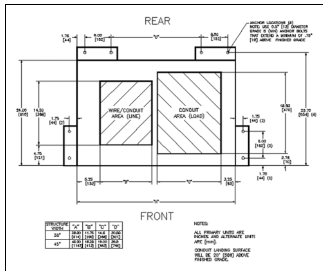
Figure 21.8-1. Bottom View Left Line (Generator) Connection
