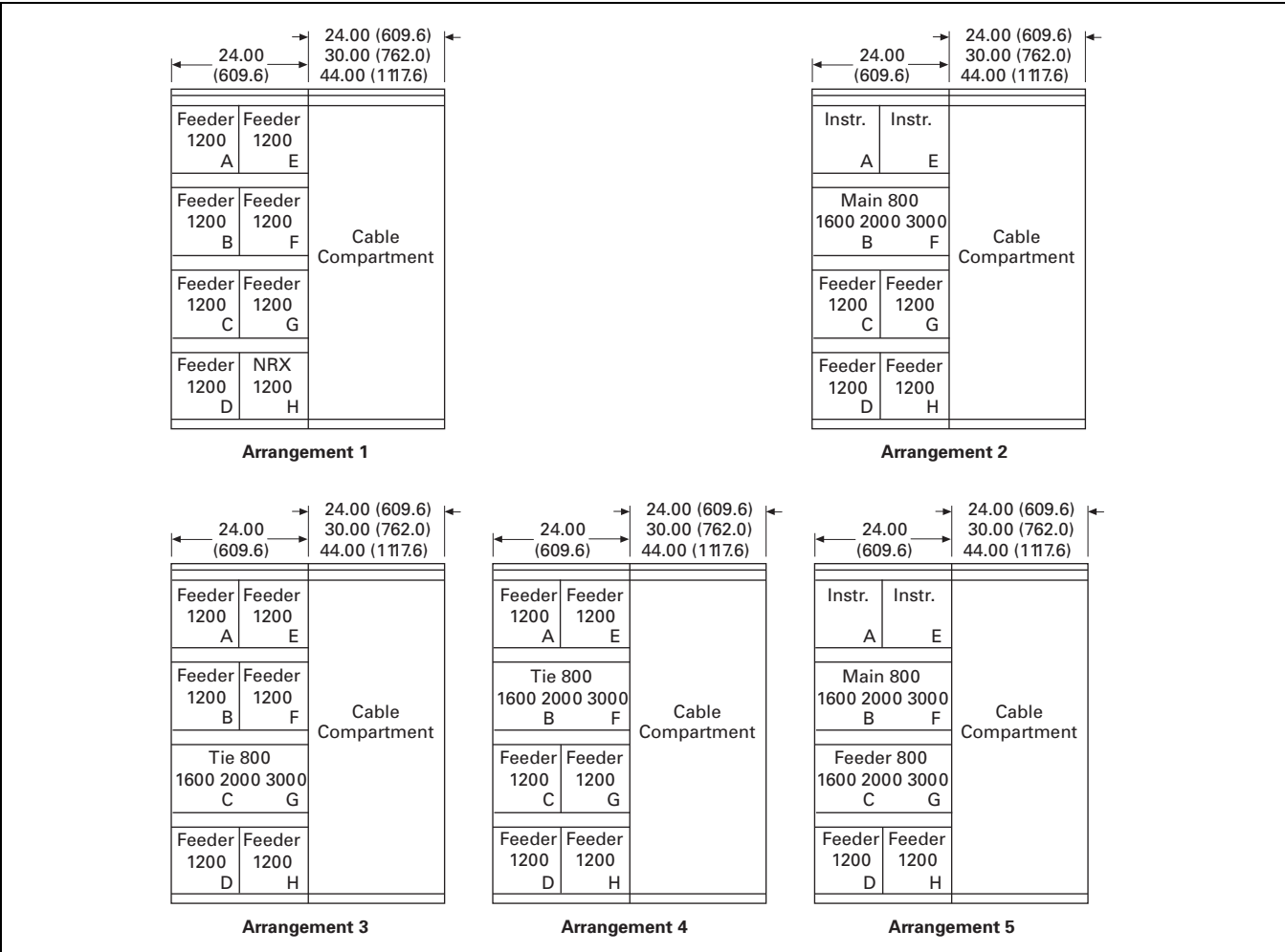
Figure 21.5-7. Typical Structure and Breaker Arrangements—Series NRX and Magnum SB Breakers
