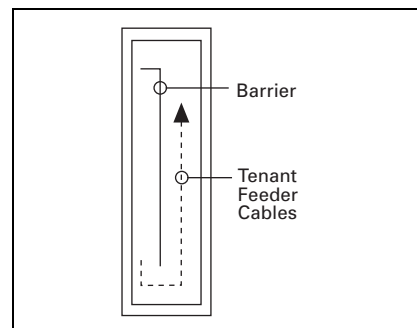
Figure 21.10-18. Rear Barrired Wireway Metering Section Side View
