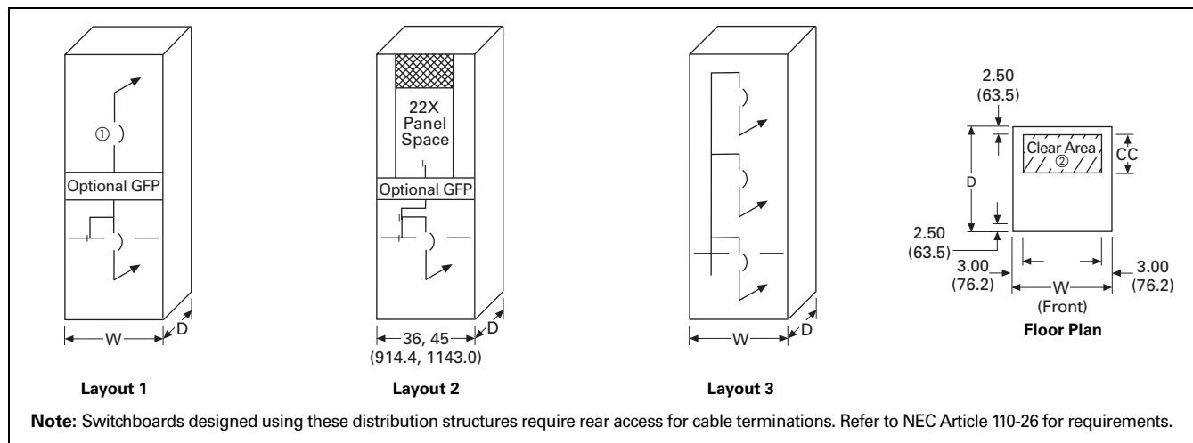
Figure 21.2-8. Individually Mounted Feeder Layouts—Dimensions in Inches (mm)
