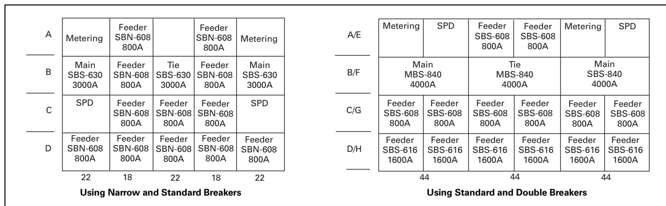
Figure 21.5-2. Main-Tie-Main Typical Layouts
