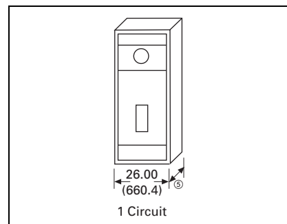
Figure 21.10-20. 400 A Tenant Section with Self-Contained Metering (Fusible Switch)
