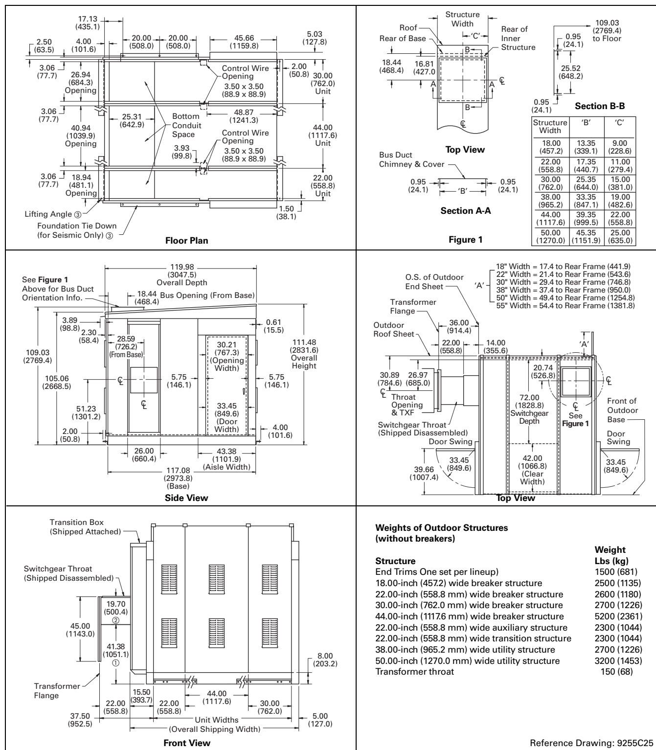
Figure 21.5-12. Outdoor Walk-in Enclosure Dimensions in Inches (mm)
