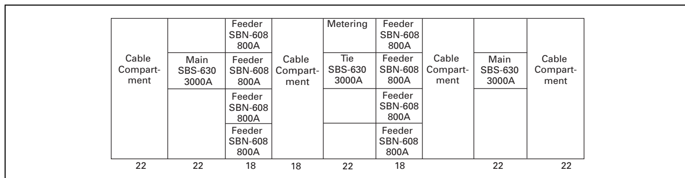
Figure 21.5-5. Standard and Narrow Breakers—Typical Main-Tie-Main Layout
