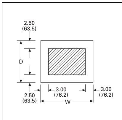
Figure 21.10-1. Typical Conduit Area—Figures 21.10-2, 21.10-3 and 21.10-4
