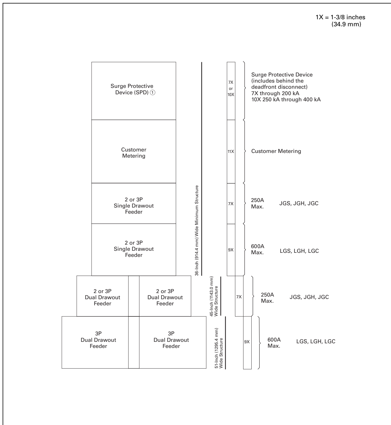
Figure 21.1-10. Circuit Breaker “X” Space Requirements—Dimensions in Inches (mm)
