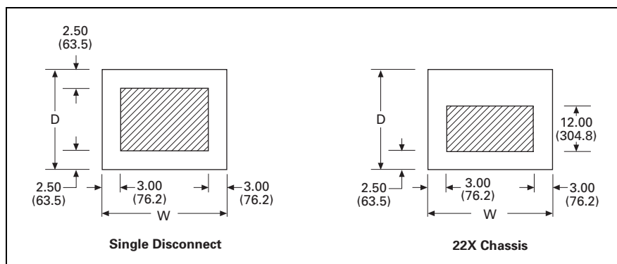
Figure 21.10-23. Typical Conduit Areas—Bottom Cable Exit
