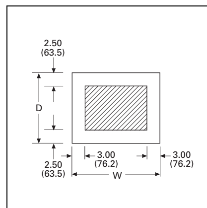
Figure 21.10-13. Typical Conduit Area—Figures 21.10-10, 21.10-11 and 21.10-12
