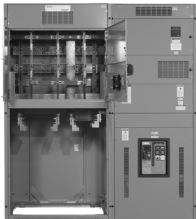
PRLC Switchboard—Front-Access
