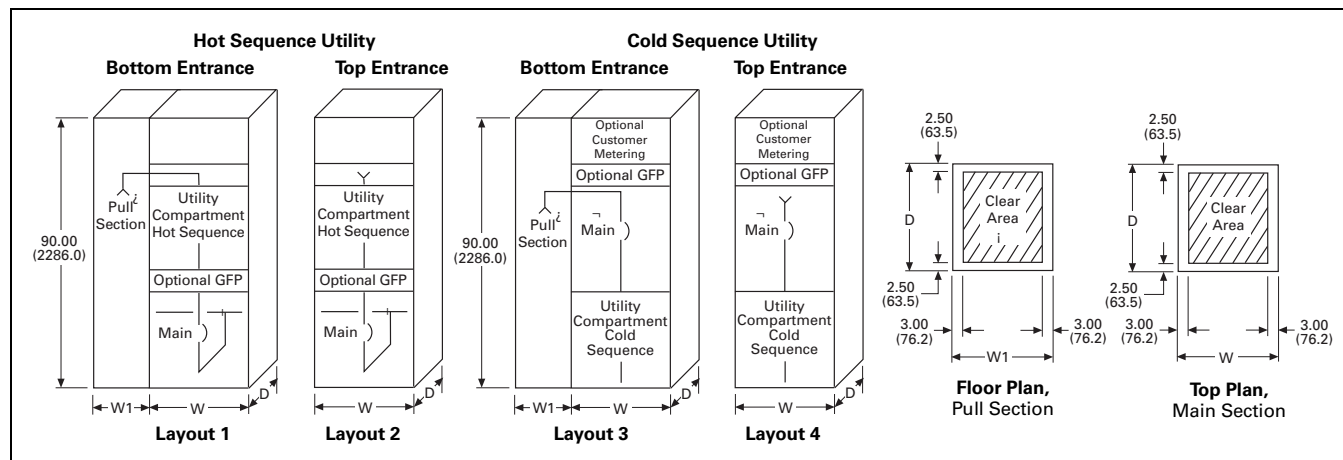
Figure 21.1-4. NEMA Utility Compartment Layouts—Dimensions in Inches (mm)
