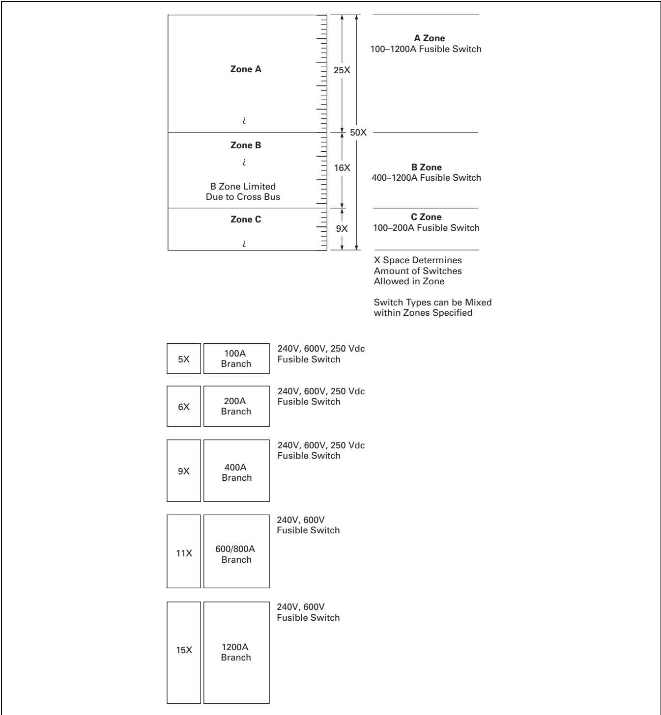
Figure 21.3-2. Individually Compartmentalized Feeder Layout 36.00-Inch (914.4 mm) Wide Section 50X Structure Only (4000 A Maximum)
