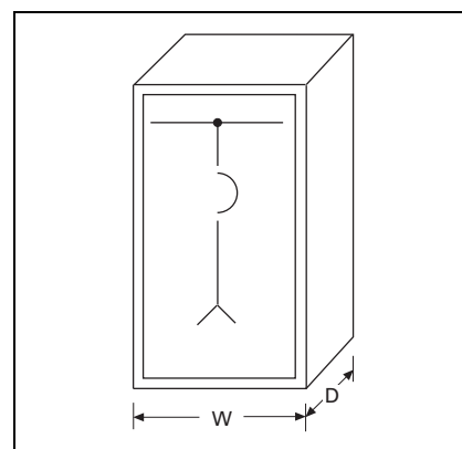
Figure 21.10-3. Main Device (Breaker or Switch)—Bottom Feed
