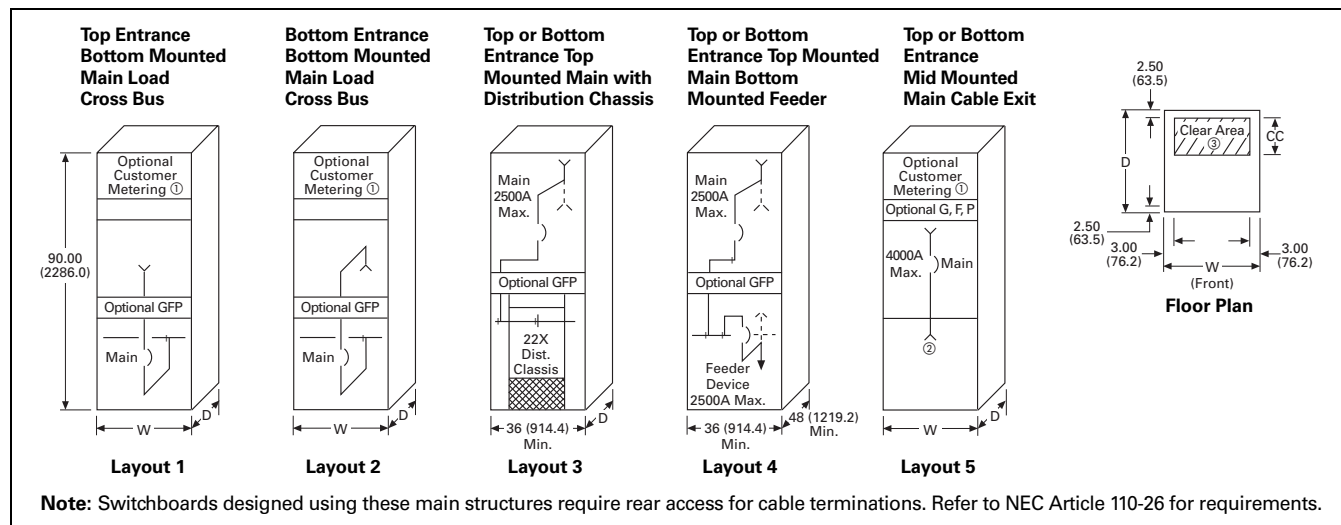
Figure 21.2-5. Main Section Layouts—Dimensions in Inches (mm)
