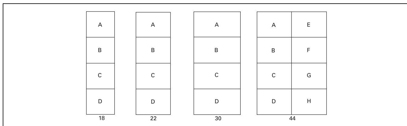
Figure 21.5-1. Breaker Structures
