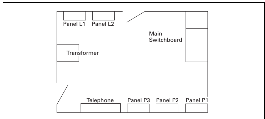
Figure 21.6-1. Traditional Electrical Room—Plan View
