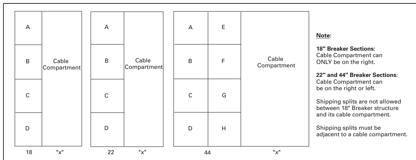
Figure 21.5-3. Breaker Structures
