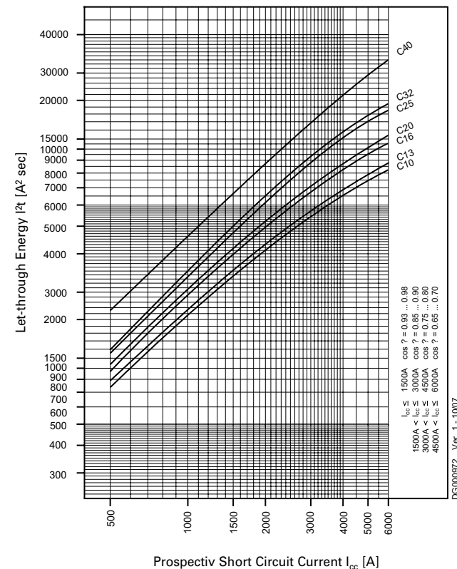
Let-through Energy FRBm6, Characteristic C, 2polig
