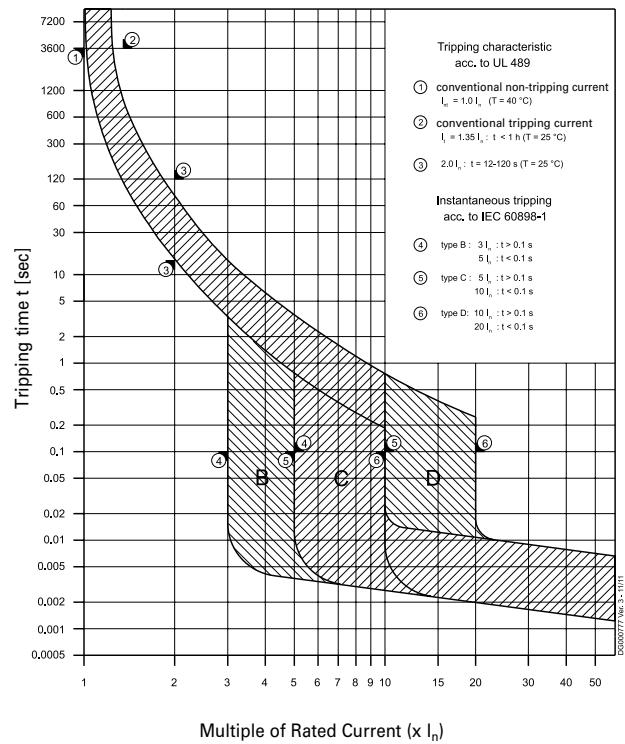
Characteristics B, C and D - UL 489
