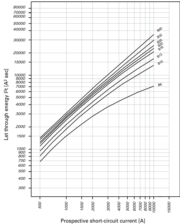
Let-through Energy FRBmM, Characteristic B, 1+Npolig
