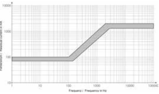
Tripping current frequency response 500 mA Type S/Bfg
