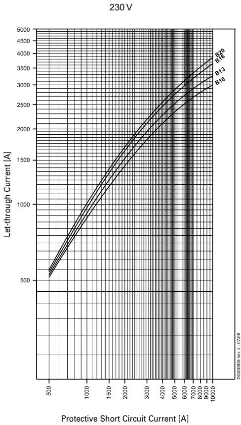
Characteristic B
