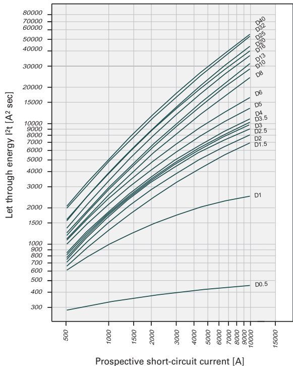
Let-through Energy mMCM, Characteristic D, 1-pole
