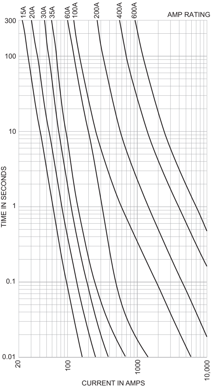
NON time-current curves — average melt
