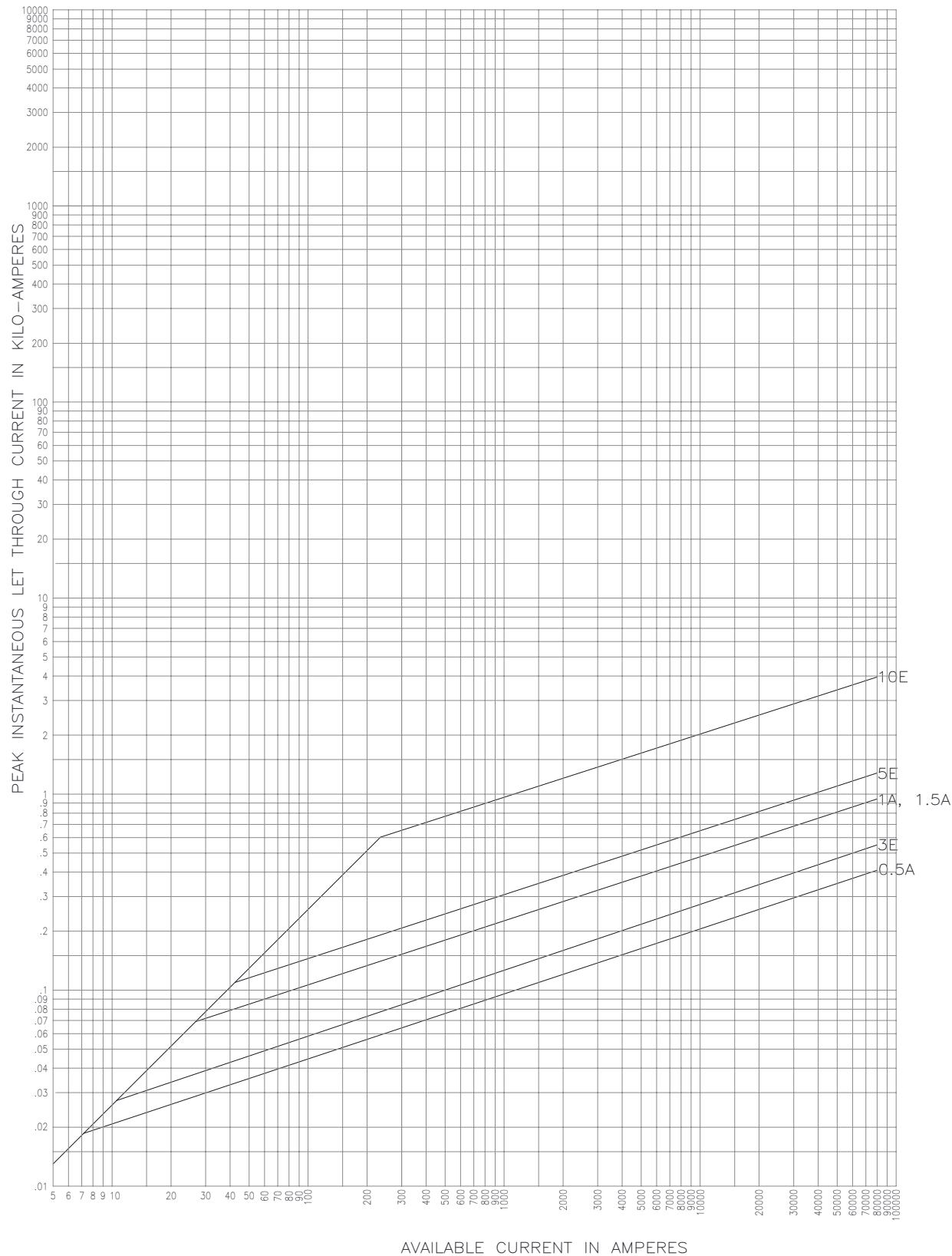
Type CLPT and JCQ Current Limiting Potential Transformer Fuses Peak Let Through Current Characteristics 15.5kV Curves are plotted to maximum test points so all variations should be negative.
