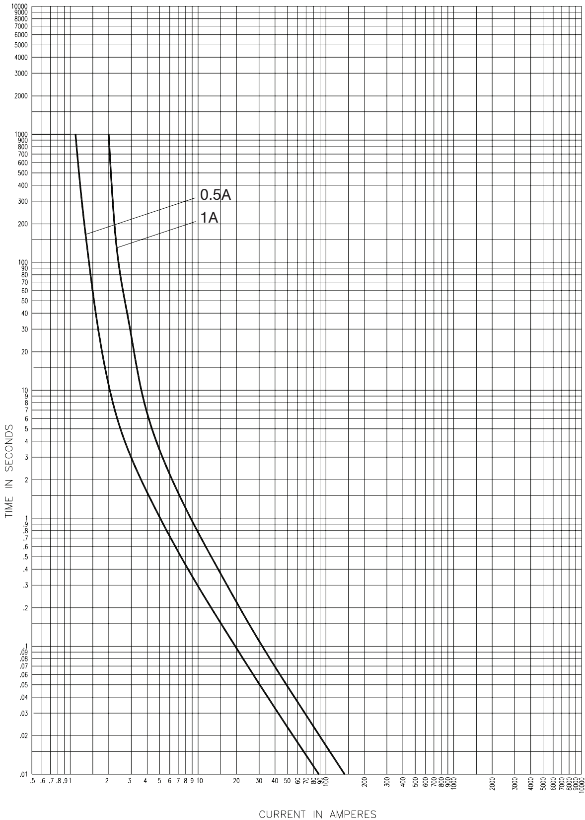
25.5kV time-current curves — total clearing for 25CLPT_
