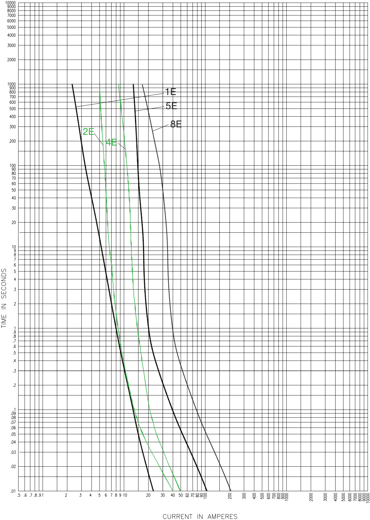
8.3kV time-current curves — total clearing for 8NCLPT_
