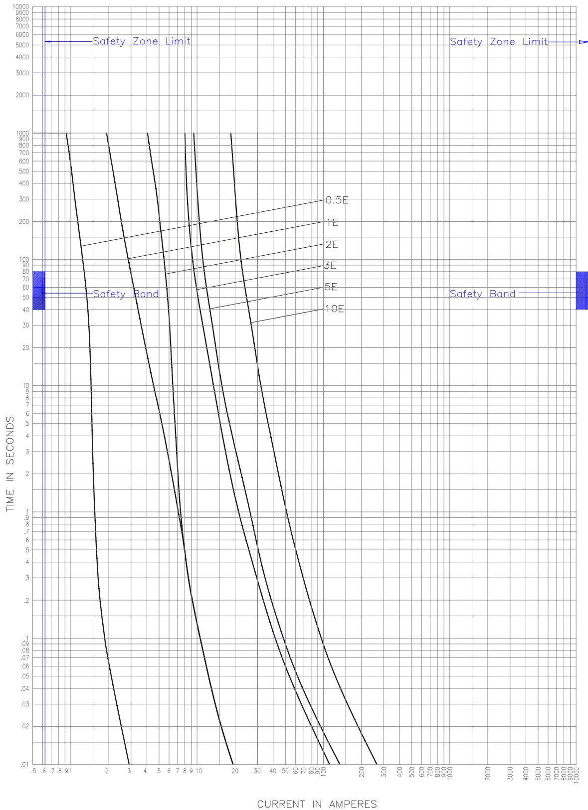
Type 5NCLPT General Purpose Current Limiting Fuses (Non-Indicating) Minimum Melting Time-Current Characteristics Curves are based on tests starting with fuse unit at ambient temperature of 25 C and without initial load. Curves are plotted to minimum test points so all variations should be positive.
