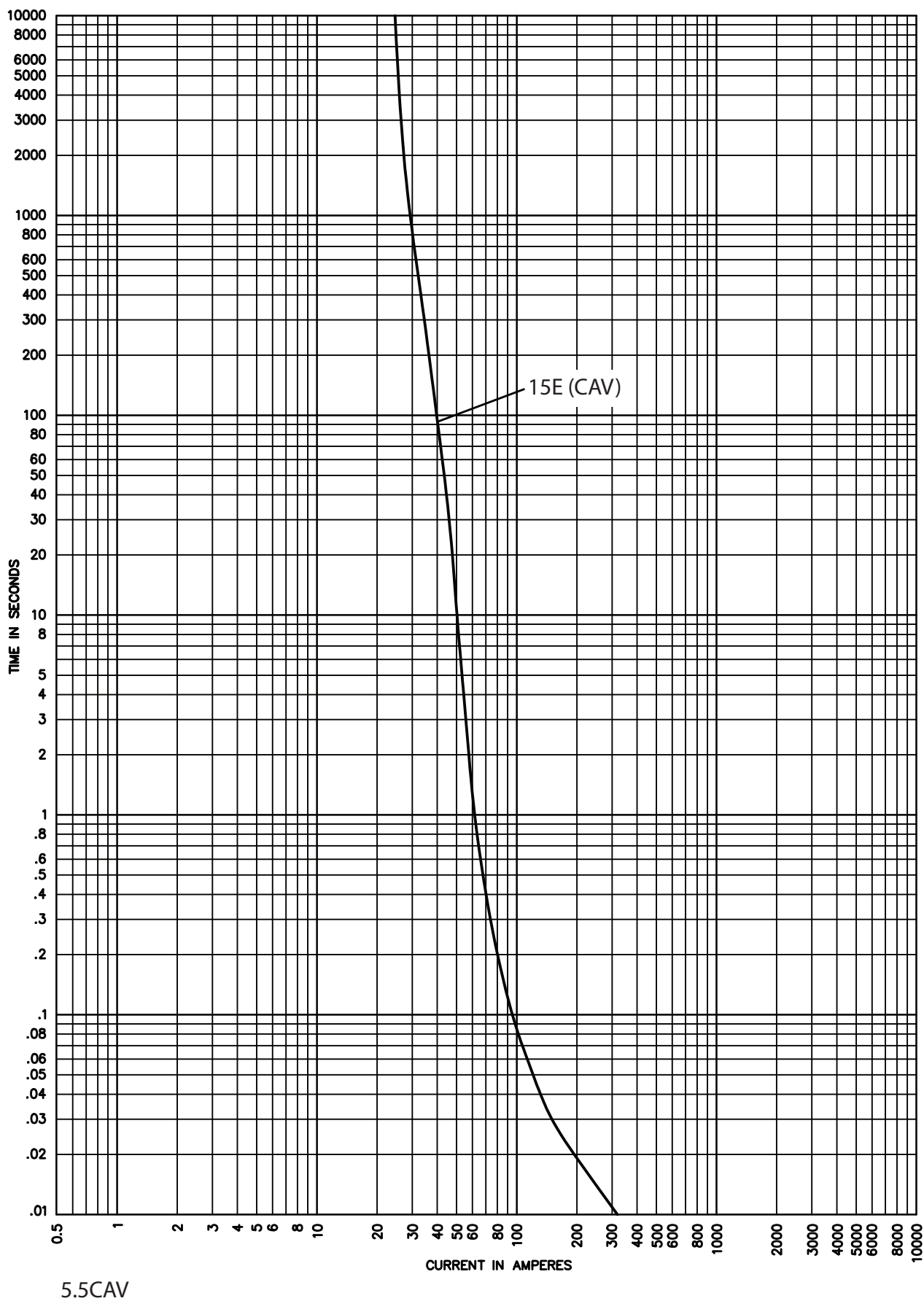
5.5kV time-current curves — total clearing for 5.5CAV_
