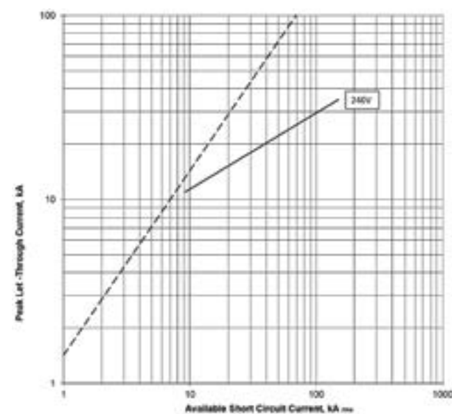
Let-through current I_D PDE2 ETU PXR10 LI; 160 A @ 240 V
