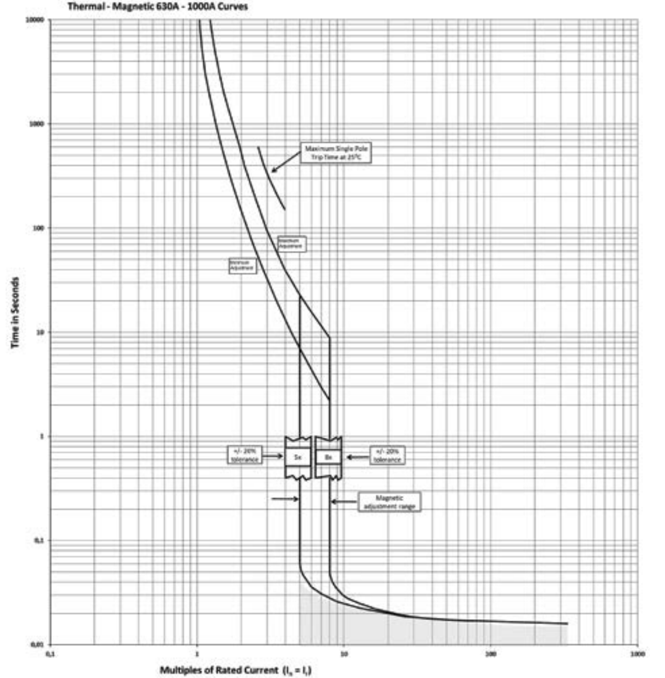
System and line protection with PDE4 TMTU; 800 A @ 240 V, 415 V and 440 V
