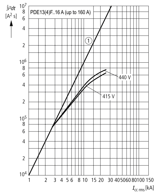
Let-through energy I^2t ; PDE1 TMTU PDE13(4)F..16 A (up to 160 A)
