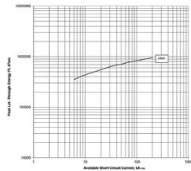
Let-through energy I^2t ; PDE2 TMTU; 250 A @ 415 V and 440 V
