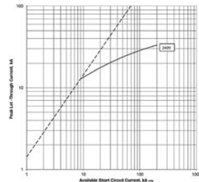
Let-through current I_D PDE2 ETU PXR10 LI; 200 A @ 240 V
