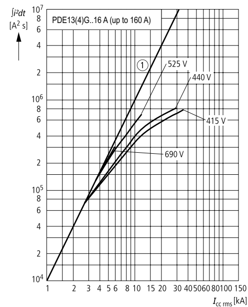
Let-through energy I^2t ; PDE1 TMTU PDE13(4)G..16 A (up to 160 A)
