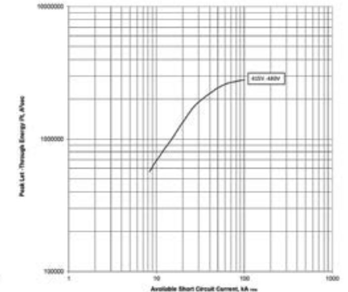
Let-through energy I^2t ; PDE9 ETU PXR10 LI; 63 A and 100 A @ 415 V and 440 V
