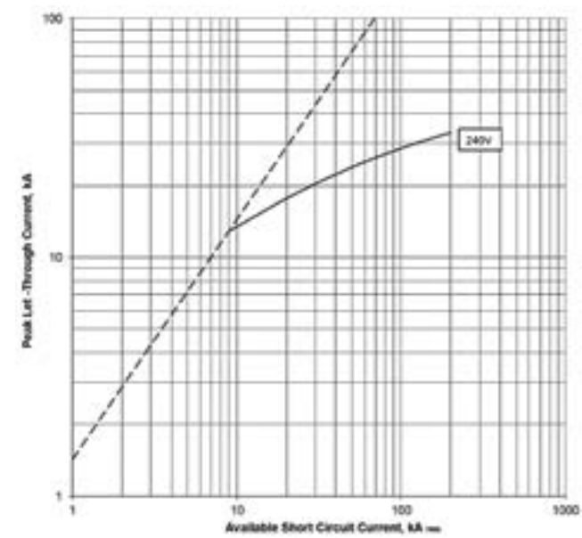
Let-through current I_D PDE2 ETU PXR10 LSI; 250 A @ 240 V
