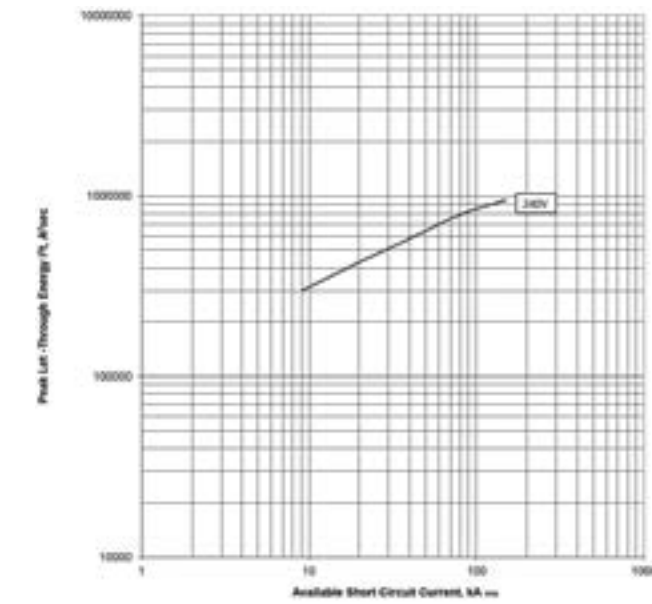
Let-through energy I^2t ; PDE2 TMTU; 160 A @ 240 V
