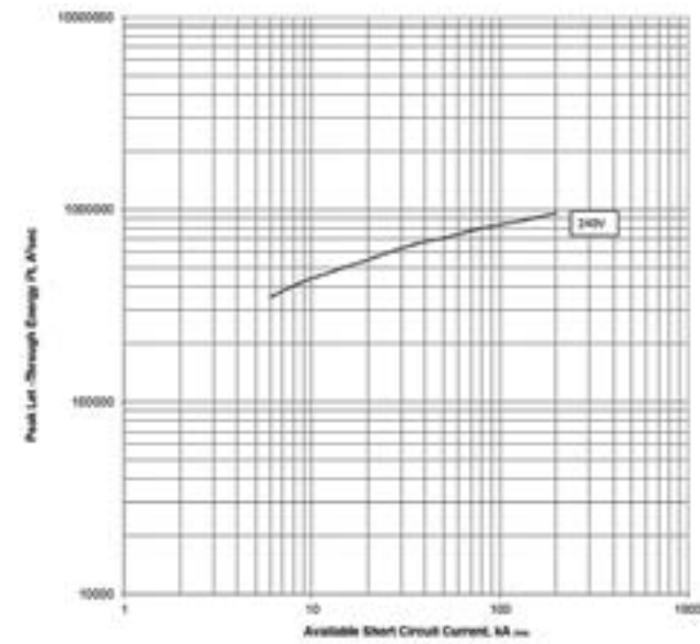
Let-through energy I^2t ; PDE2 TMTU; 200 A @ 240 V
