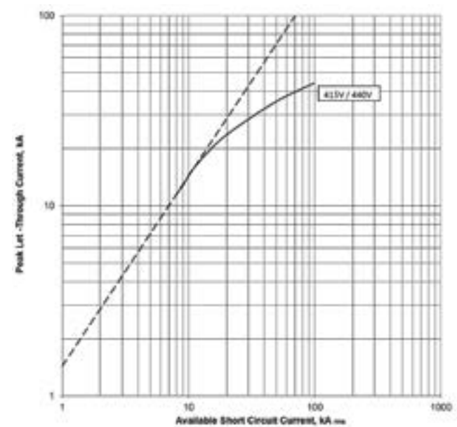
Let-through current I_D PDE2 ETU PXR10 LSI; 250 A @ 415 V and 440 V
