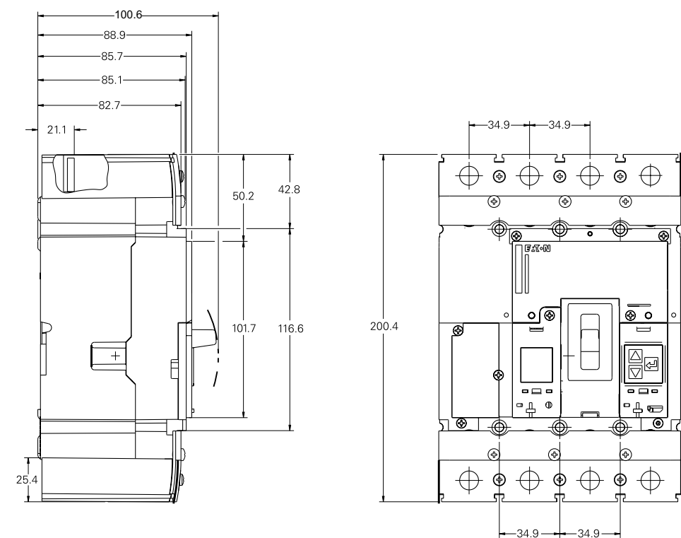
Circuit-Breakers, 4 pole (160 - 250 A)
