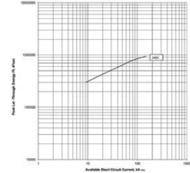
Let-through energy I^2t ; PDE2 ETU PXR10 LSI; 100 A and 160 A @ 240 V
