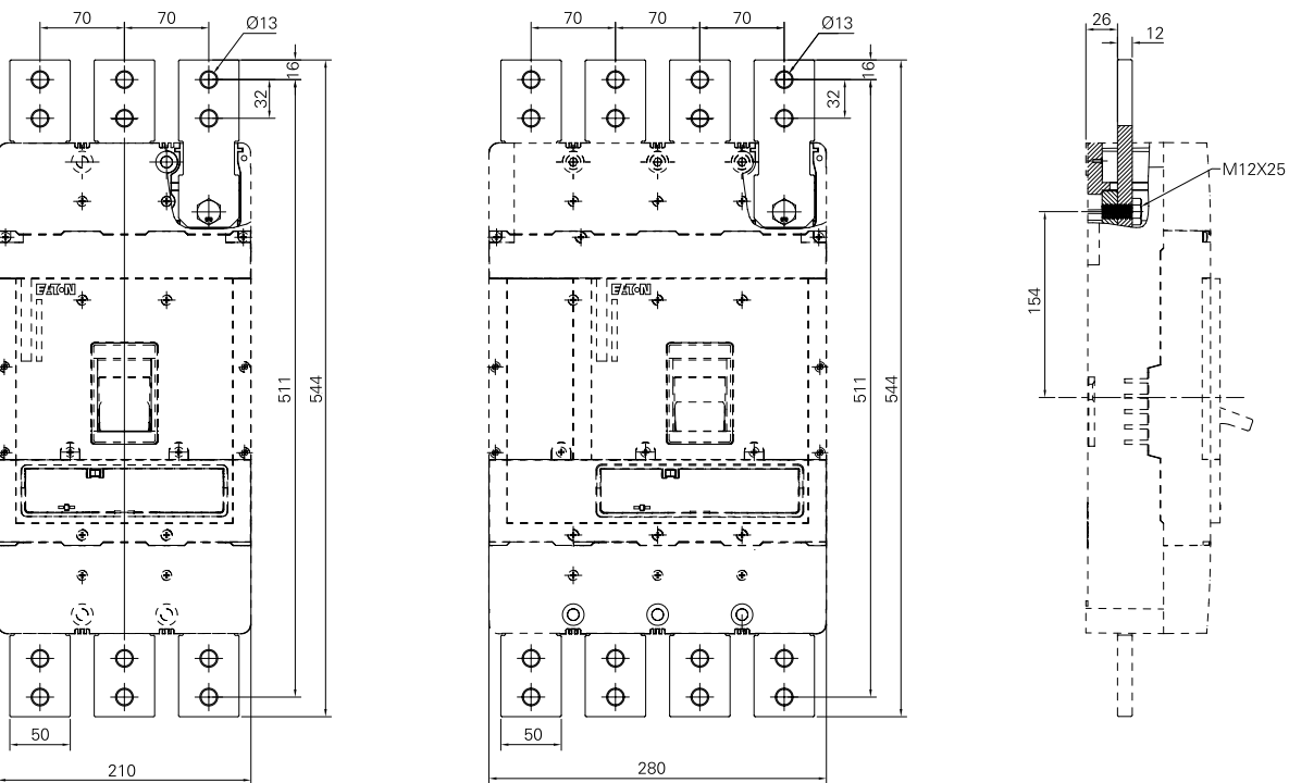
Terminal spreaders 2
