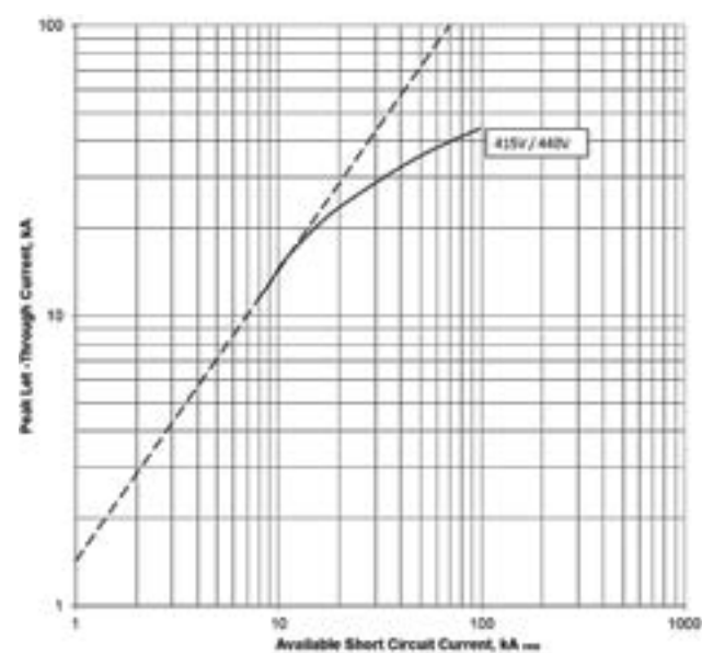
Let-through current I_D PDE2 TMTU; 250 A @ 415 V and 440 V
