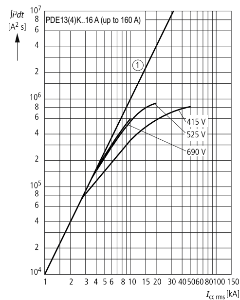
Let-through energy I^2t ; PDE1 TMTU PDE13(4)K..16 A (up to 160 A)
