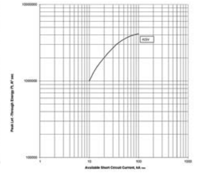
Let Through energy I^2t ; PDE3 ETU PXR10 LI; 400 A @ 415 V
