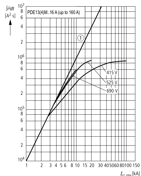
Let-through energy I^2t ; PDE1 TMTU PDE13(4)M..16 A (up to 160 A)
