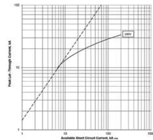
Let-through current I_D PDE2 ETU PXR10 LI; 250 A @ 240 V
