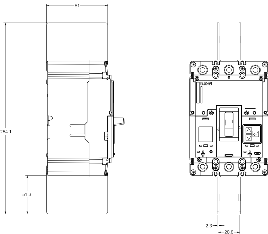
Interphase Barriers (63 - 160 A)
