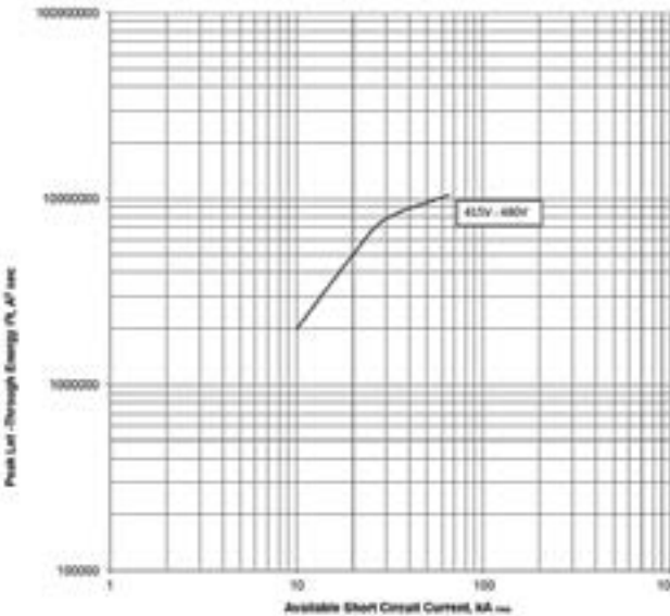
Let-through energy I^2t ; PDE4 TMTU; 800 A @ 415 V and 440 V
