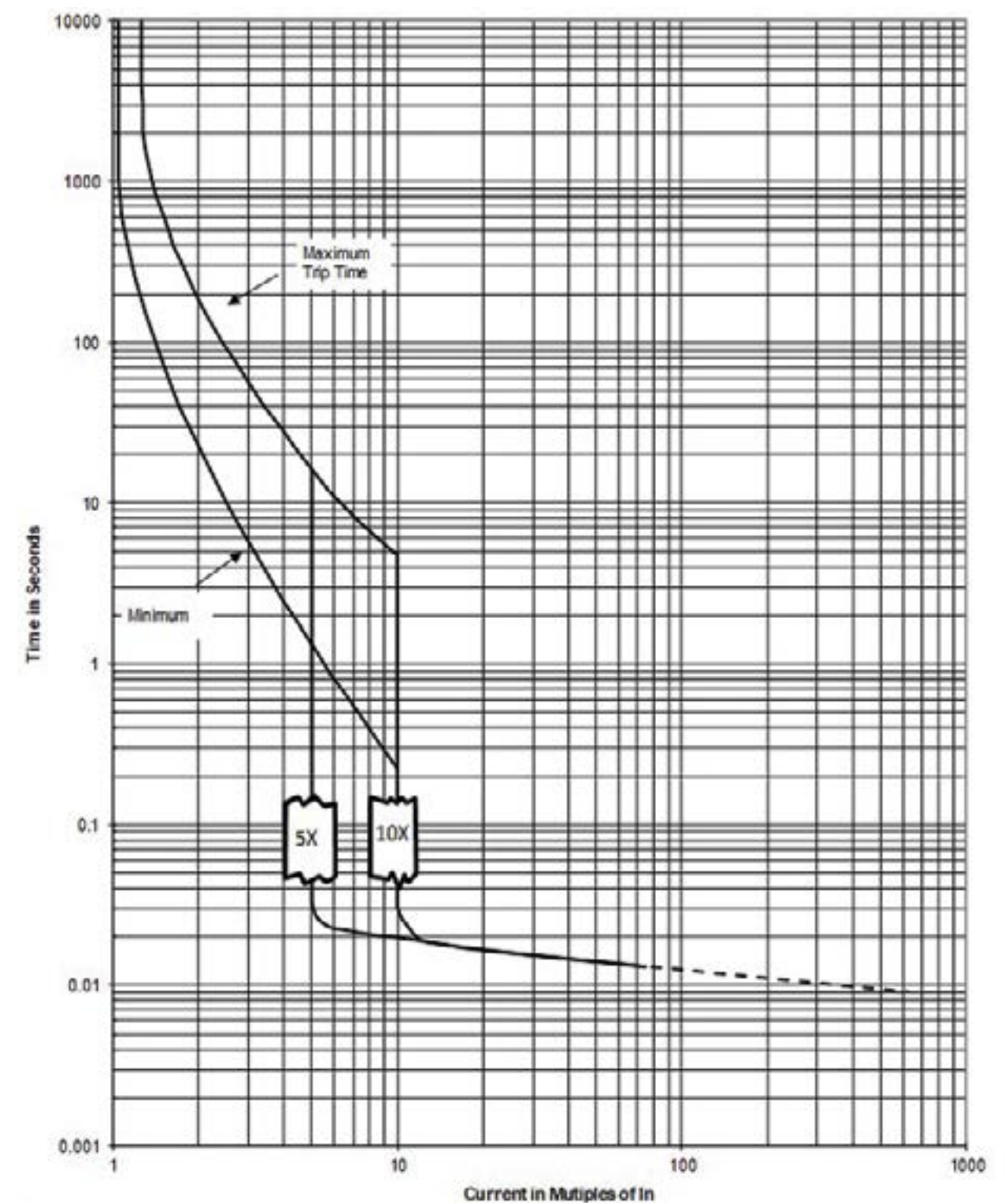
System and line protection with PDE2 TMTU; 160 A, 200 A and 250 A @ 240 V, 415 V and 440 V
