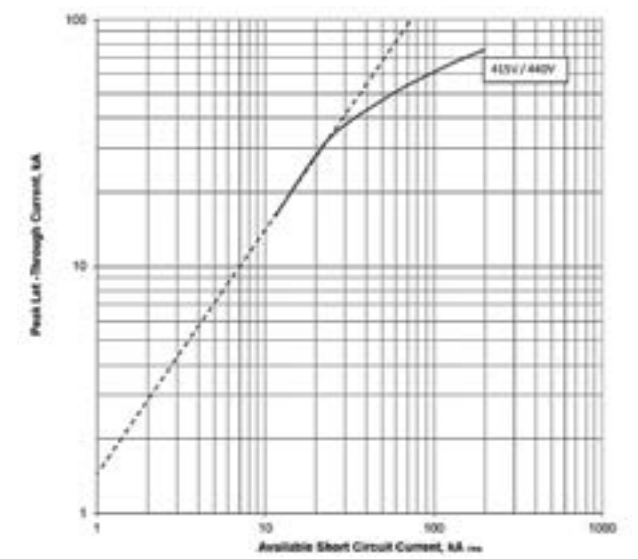
Let-through current I_D ; PDE3 TMTU; 500 A and 630 A @ 415V and 440V
