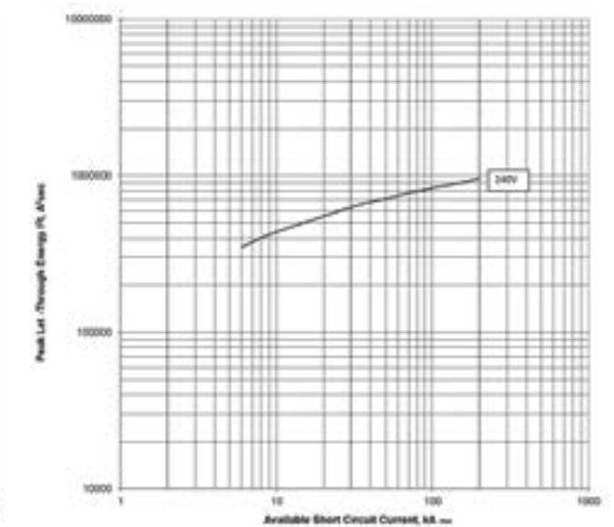
Let-through energy I^2t ; PDE2 ETU PXR10 LI; 200 A @ 415 V and 440 V
