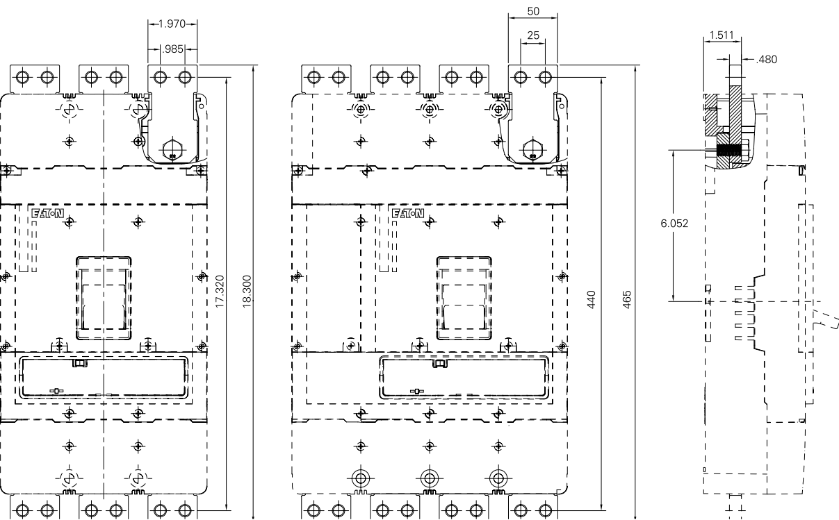
Terminal spreaders 2
