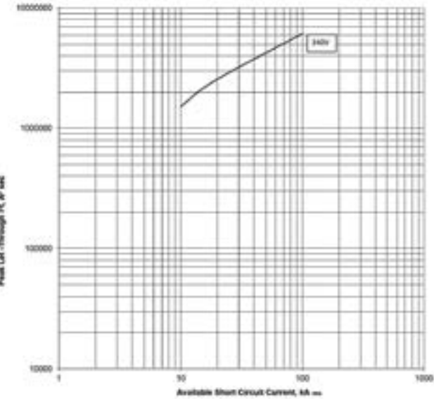
Let-through energy I^2t ; PDE4 TMTU; 800 A @ 240 V
