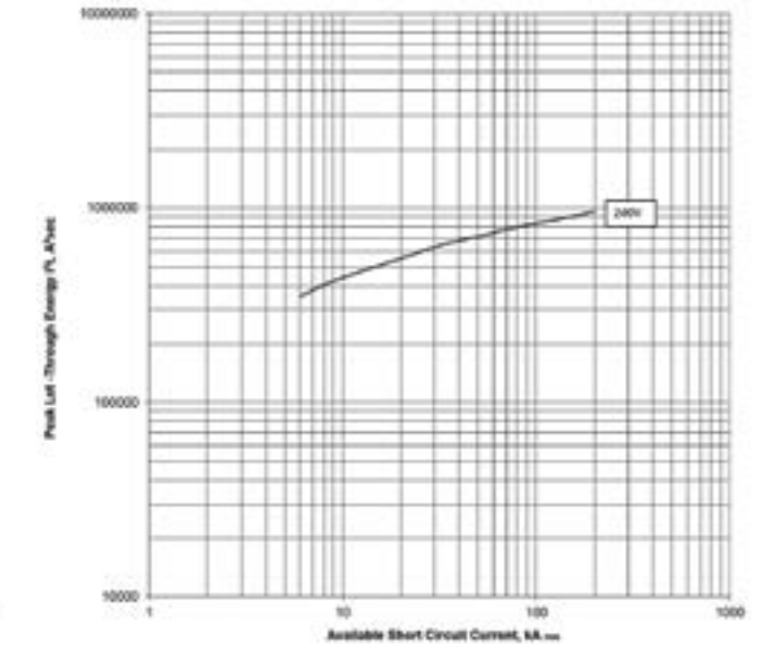
Let-through energy I^2t ; PDE2 ETU PXR10 LSI; 220 A @ 415 V and 440 V
