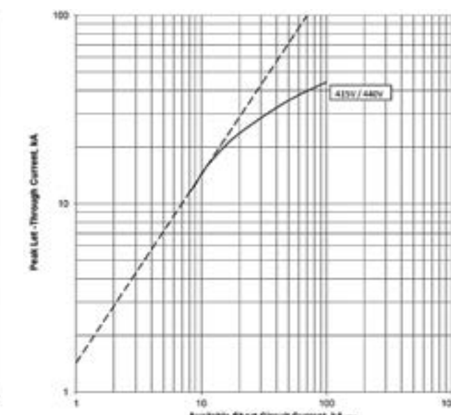
Let-through current I_D PDE2 ETU PXR10 LI; 200 A @ 415 V and 440 V
