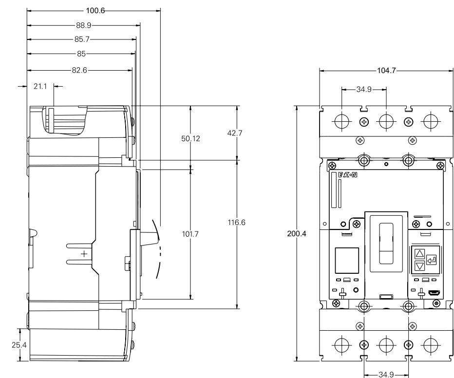
Frame size 2 Circuit-Breakers, 3 pole (160 - 250 A)
