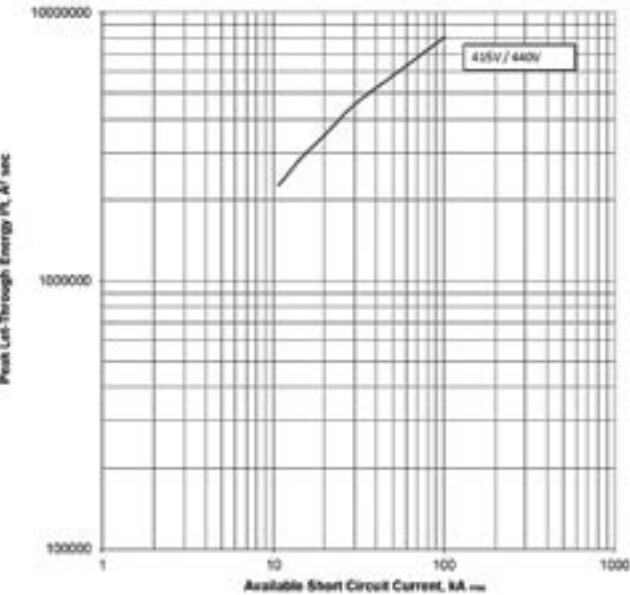
Let Through energy I^2t ; PDE3 ETU PXR10 LI; 630 A @ 415V and 440V
