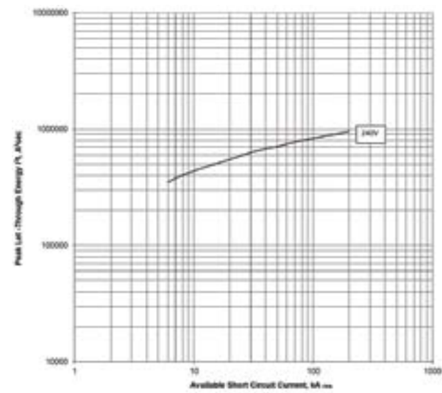
Let-through energy I^2t ; PDE2 TMTU; 250 A @ 240 V
