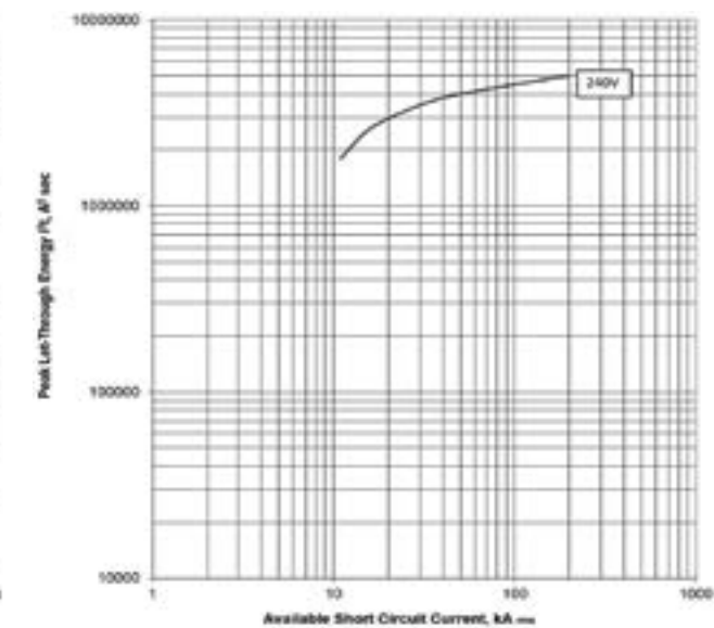
Let Through energy I^2t ; PDE3 ETU PXR10 LI; 630 A @ 240 V
