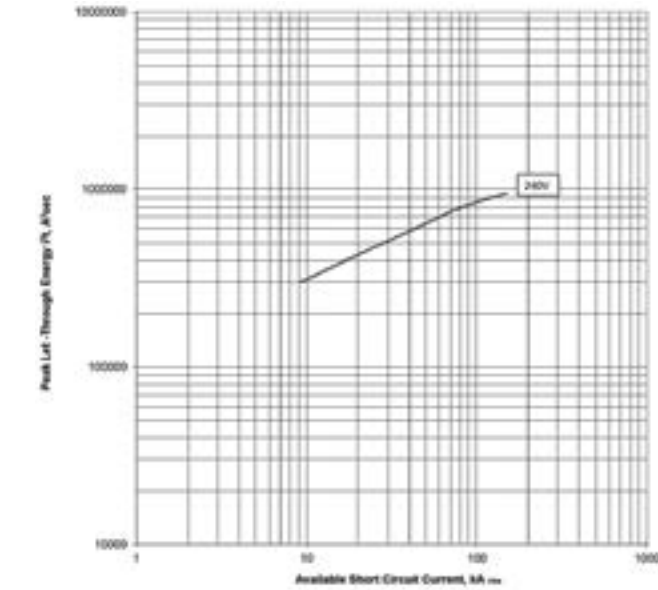
Let-through energy I^2t ; PDE9 ETU PXR10 LI; 63 A and 100 A @ 240 V
