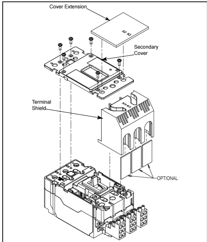
Fig. 2-1 Load Terminal Shield Kit installation layout
