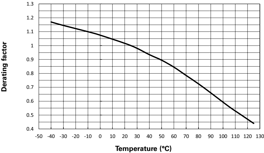
Temperature derating curve
