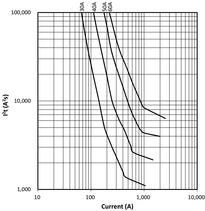
I²t vs. current curve
