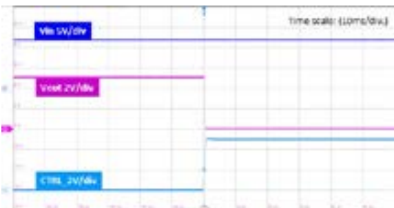
Figure 7: CNTRL high level, DC-DC off
