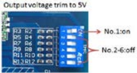
Figure 4: 5 V trimming output example
