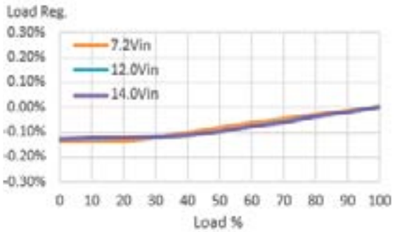
Load regulation vs. load
