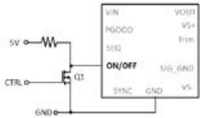
Figure 5: Remote on/off circuit diagram
