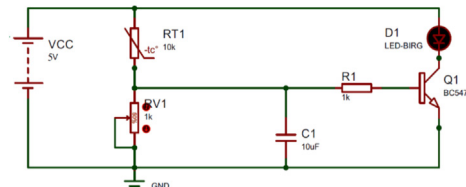
Figure 8. Thermistor-based thermostat circuit diagram
