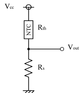
Figure 6. Basic circuit diagram for thermistor linearization
