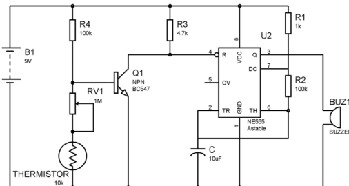
Figure 9. Thermistor-based fire alarm circuit
