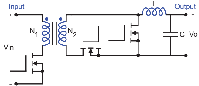
Figure 2. Forward topology
