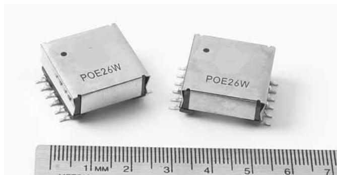
Figure 4. Eaton's 26 W forward converter transformers
