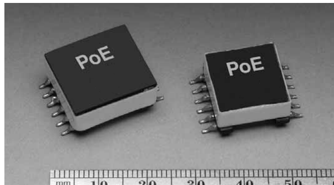
Figure 3. Eaton's 4 W to 13 W flyback transformers
