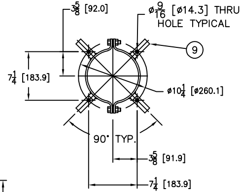
MOUNTING DETAIL
