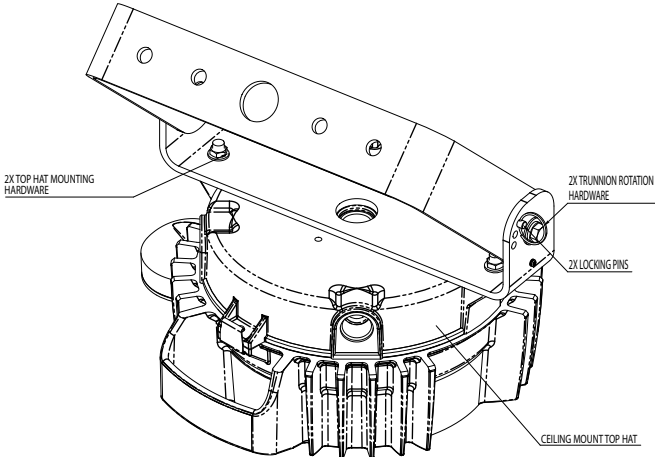
Trunnion
