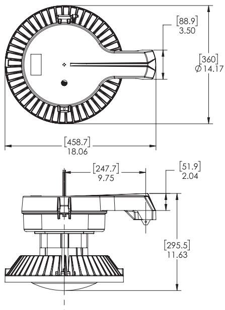
Stanchion - straight
