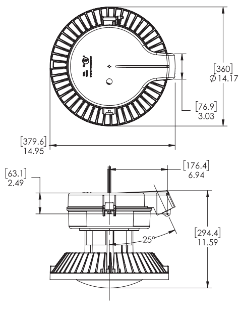
Stanchion - 25° angled
