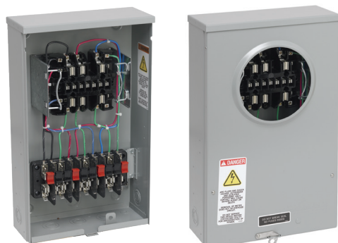
SW02132S1GR1N shown open & closed
