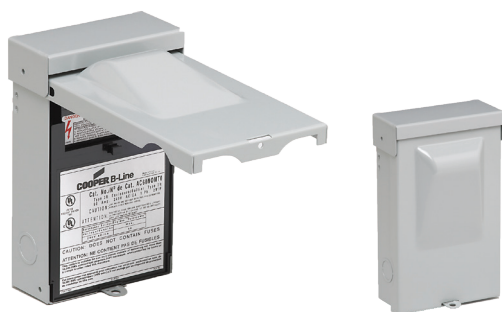
AC60NOMT0 shown open & closed
