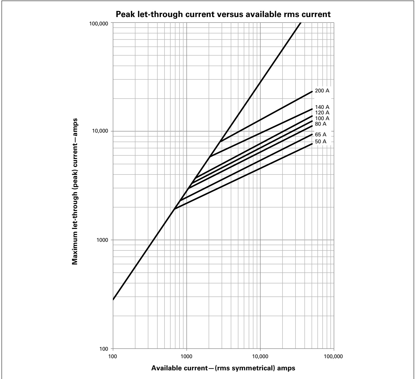
Figure 4. Peak let-through curves for 38 kV ELSP backup current-limiting fuse
