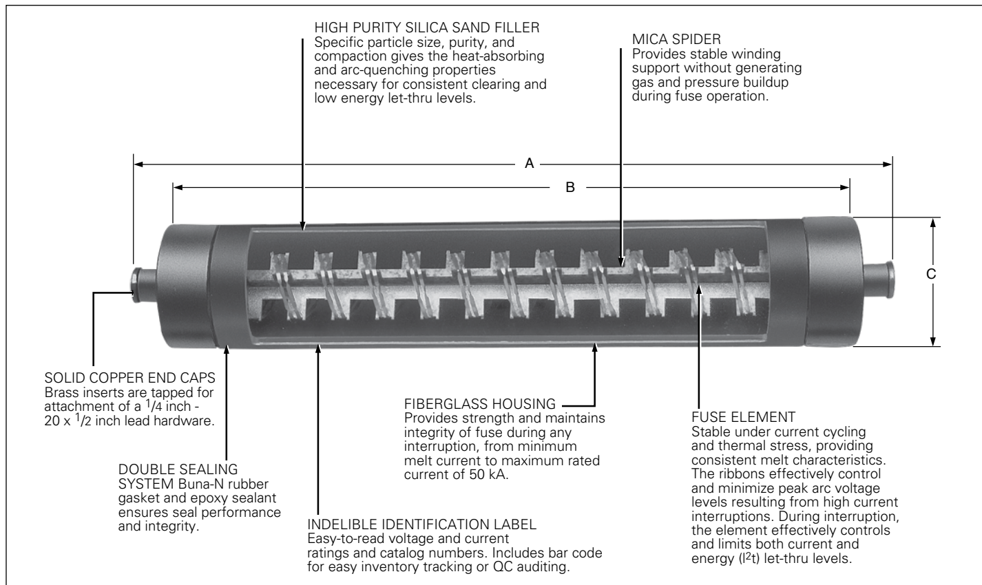
Figure 1. 2 inch diameter ELSP current-limiting backup fuse cutaway shows design characteristics
