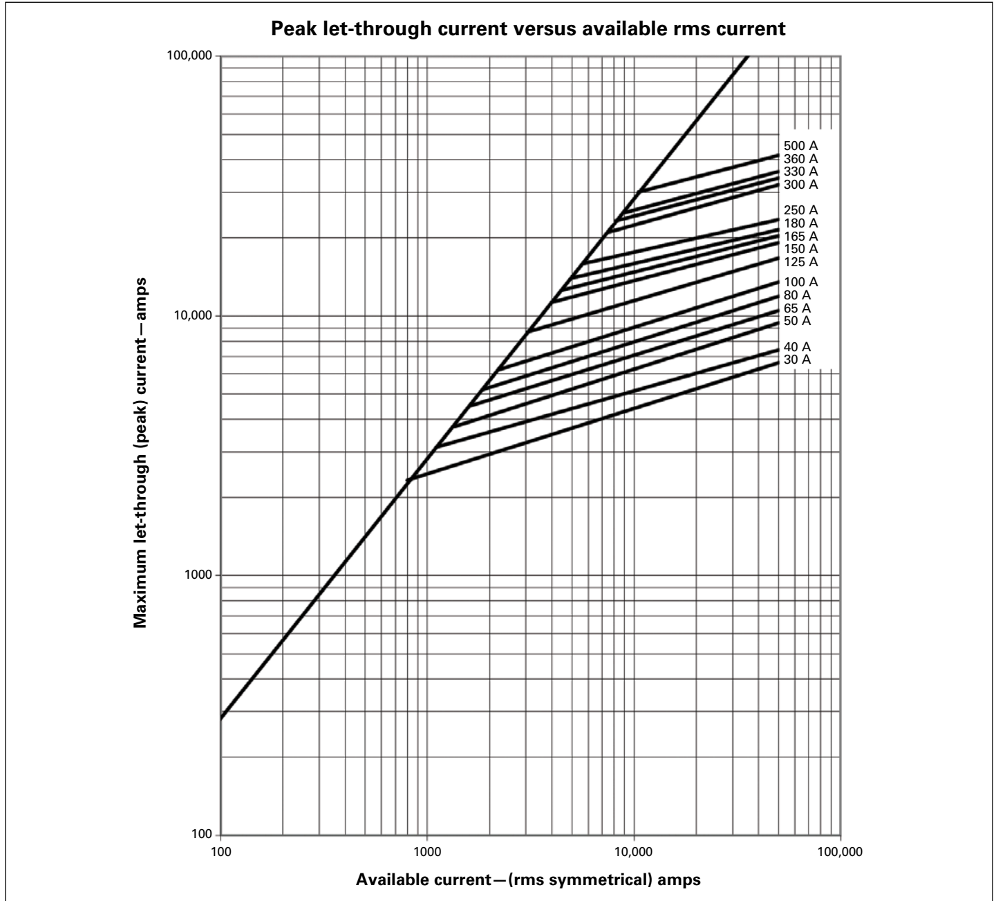
Figure 3. Peak let-through curves for 8.3 kV, 9.9 kV, 15.5 kV, 17.2 kV, and 23 kV ELSP backup current-limiting fuse
