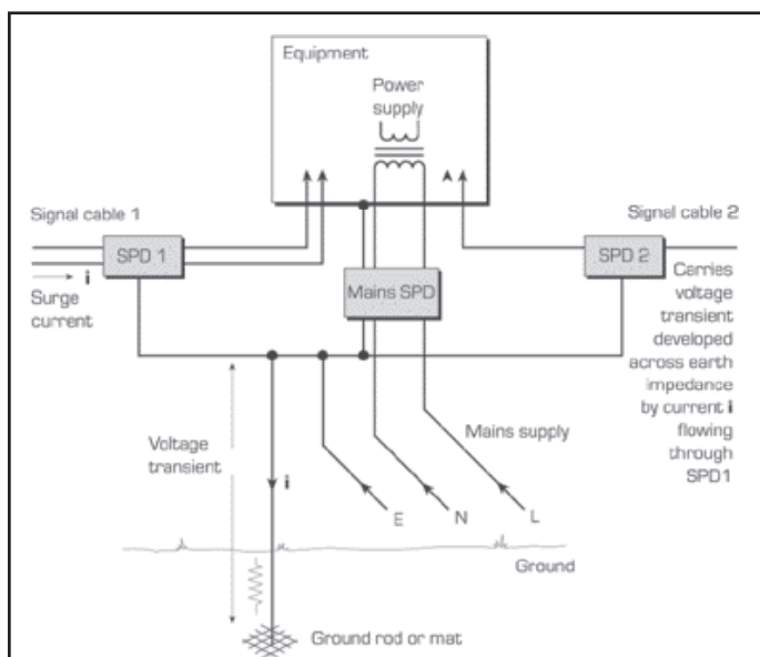
Figure 35 Advantages of low ground impedance
