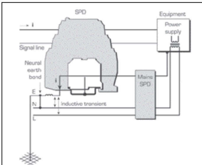
Figure 29 Preventing surge coupling having adverse effects
