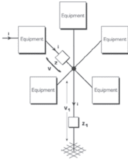
Figure 23 Current flow through one device in a star-point earth system
