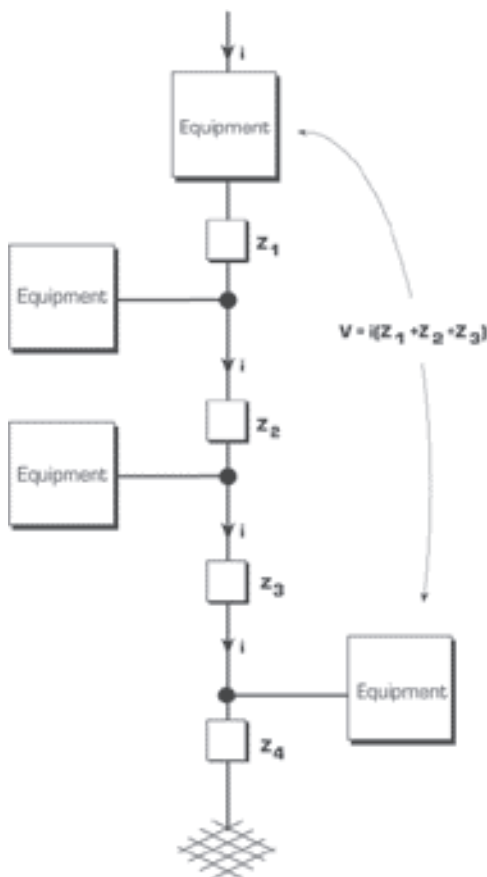
Figure 24 Vagaries of an earth system with variable connections to a common earth connection
