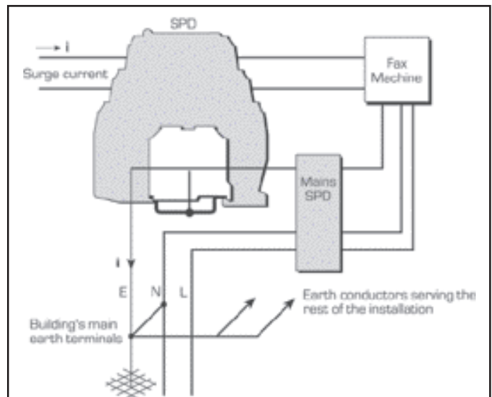
Figure 31 An example of relatively isolated equipment
