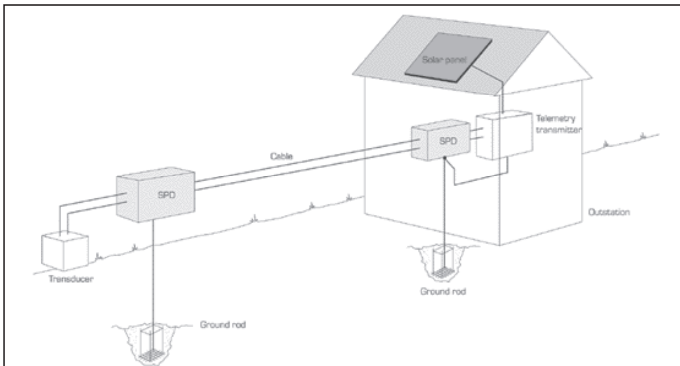
Figure 34 Outstation installation – with ground rod
