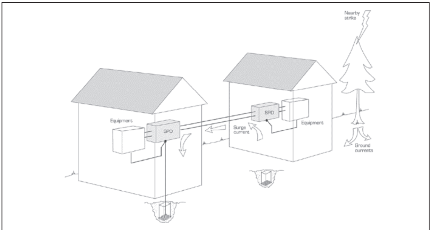
Figure 37 Bonding a structural lightning protection system to the system star-point
