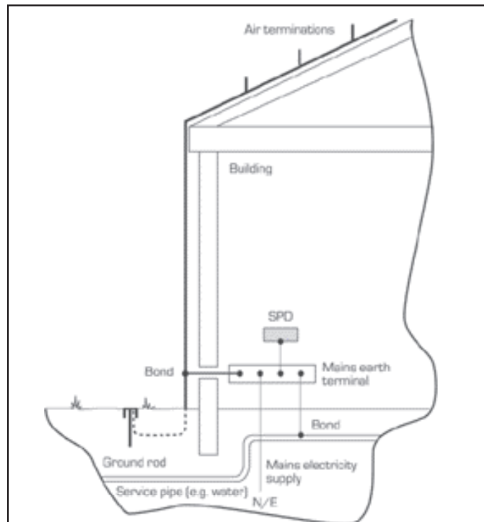
Figure 36 Bonding a structural lightning protection system to the system star-point
