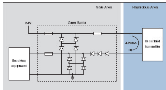
Figure 1: Typical intrinsically safe 4-20mA transmitter loop
