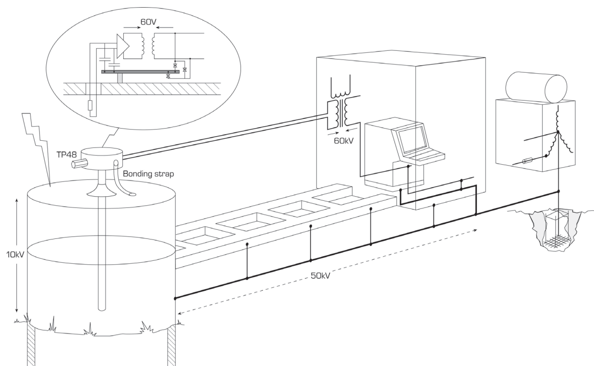
Figure 4 Intrinsically safe circuit fully protected
