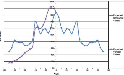
Figure 6: Light Distribution
