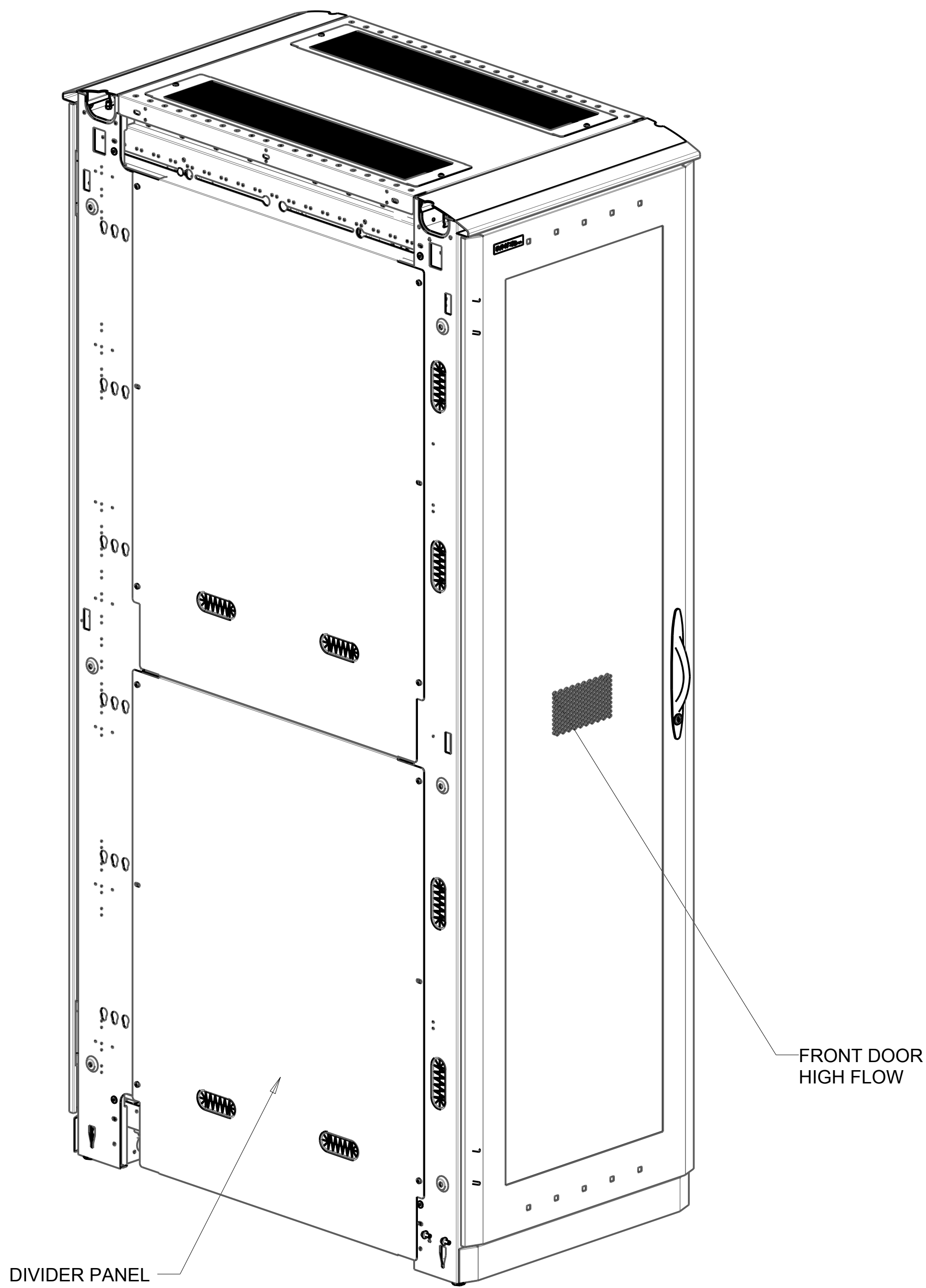
FRONT ISO
