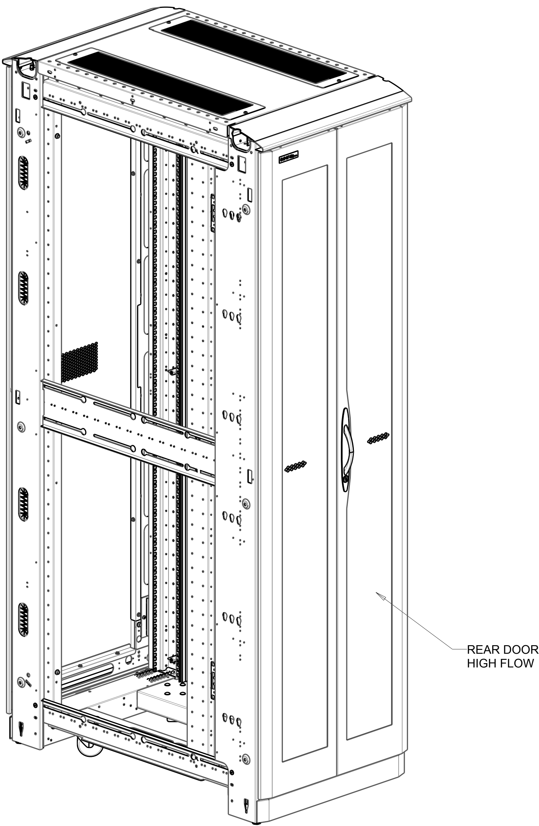
REAR ISO
