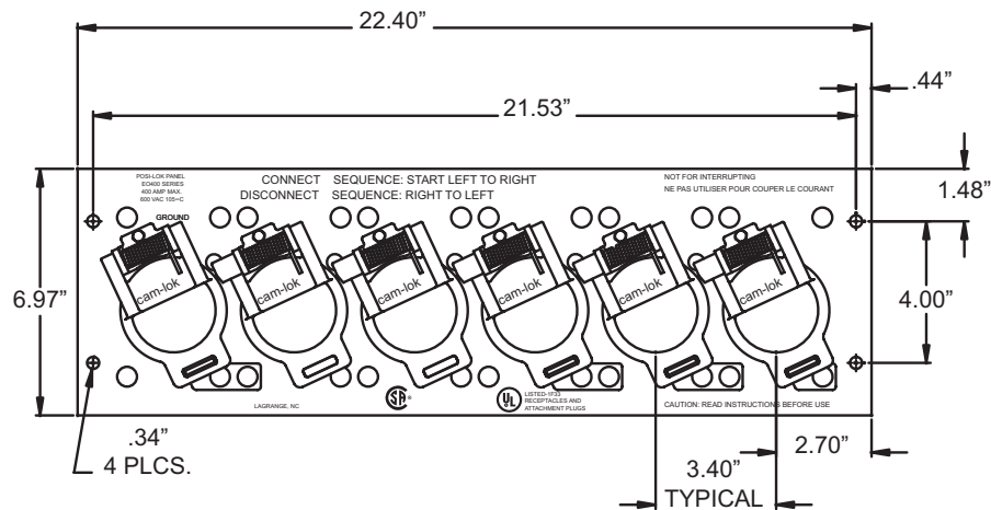
Panel without limit switch mounting dimensions
