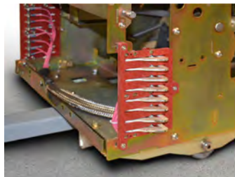
Utility Grade Secondary Disconnect
