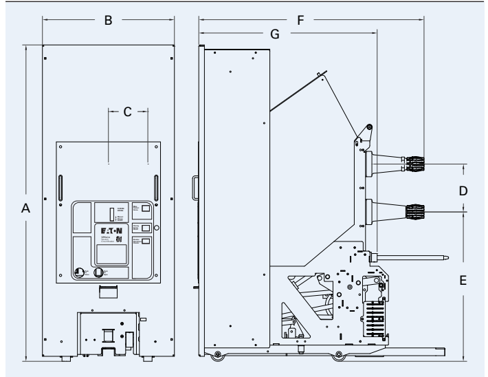
Dimensional Data In Inches
