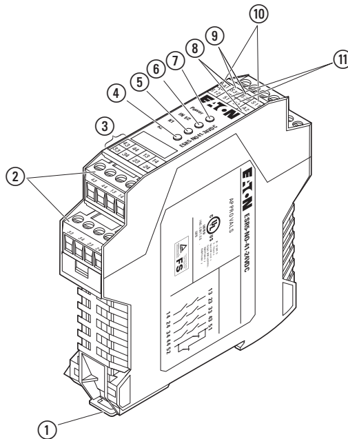
Figure 1: ESR5-NO-41-24VDC
