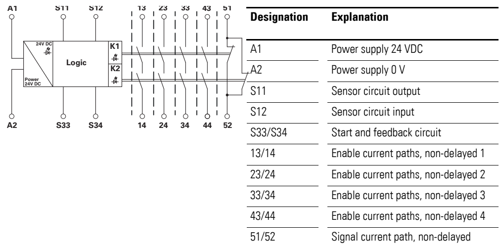
Figure 4: Block diagram
