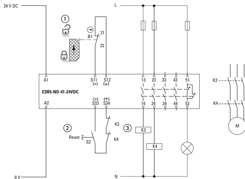
Figure 12: Single-channel protective door monitoring / manual start
