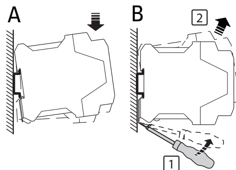
Figure 8: Mounting A and disassembly B
