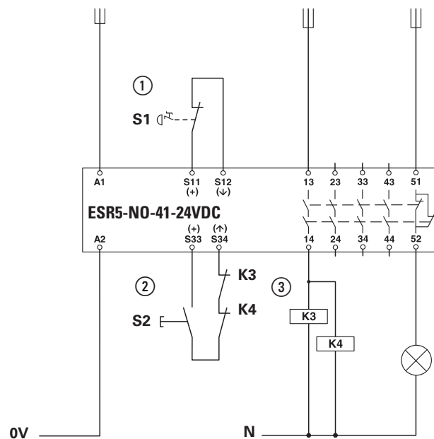
Figure 13: Single-channel EMERGENCY STOP monitoring / manual start
