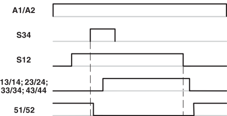
Figure 3: Time diagram manual start
