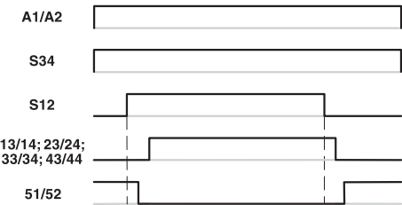
Figure 2: Time diagram automatic start
