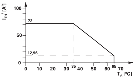
Figure 5: Derating curve – vertical and horizontal mounting positions, without distance
